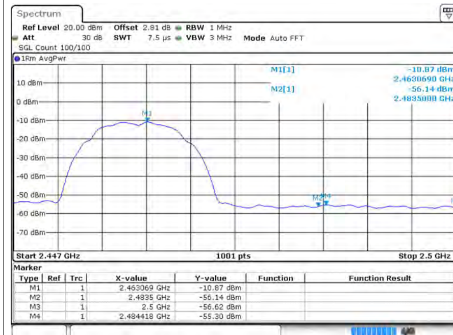
b 2462MHz Ant1 Average
