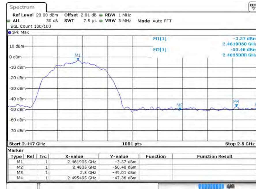
b 2462MHz Ant1 Peak
