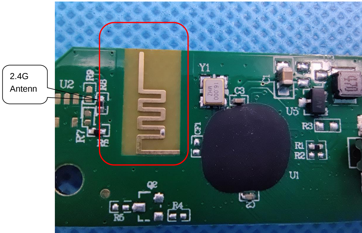
INTERNAL VIEW OF EUT (FIGURE 3)
