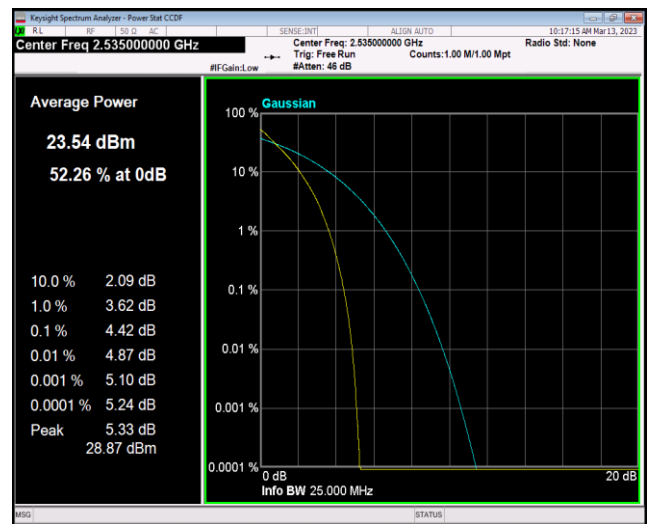
Band7-20MHz-64QAM-21100-100RB#0
