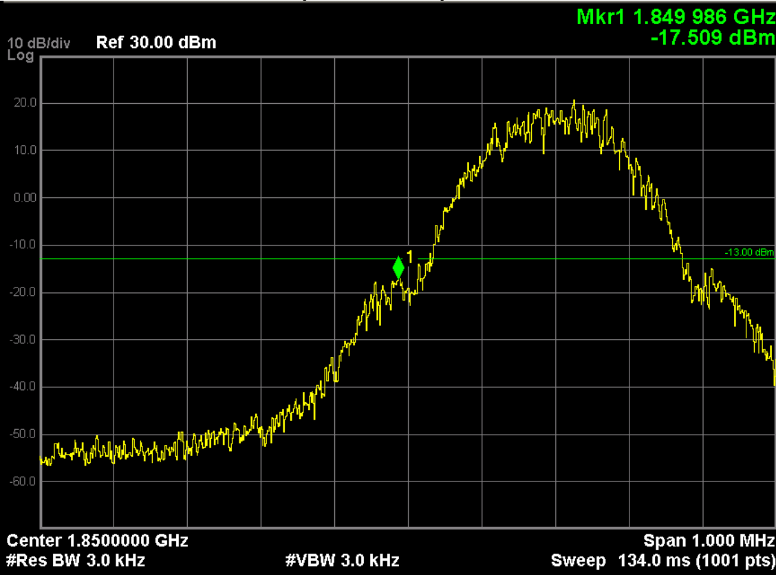
GSM1900 (EGPRS 8 Link), Channel 512
