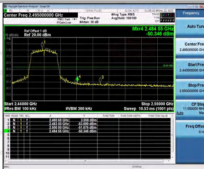
802.11n(HT20)SISO_Ant2_High_2462
