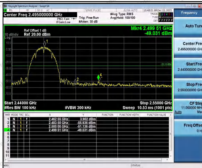
802.11b_Ant2_High_2462
