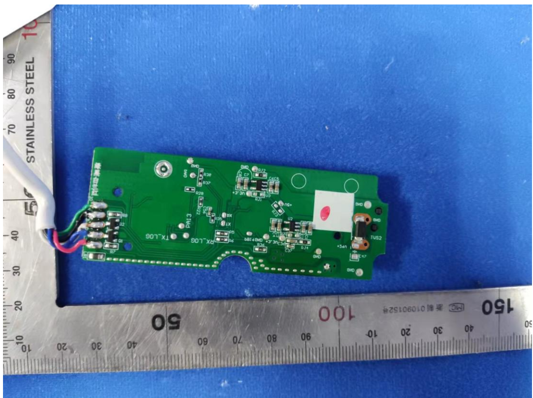
FIGURE 5 CYNC DIRECT CONNECTED INDOOR PREMIUM LIGHT STRIP (16FT.) (M/N: CLEDSTR24CDIDP) MAINBOARD FRONT
