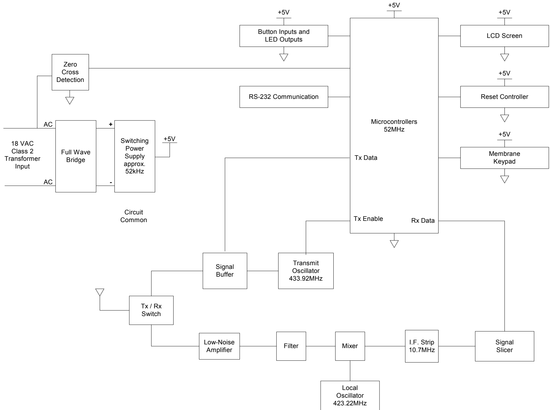
RB-SBT Block Diagram (JPZ0027)
