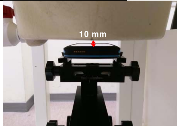
Fig.7 EUT Front side to flat phantom
