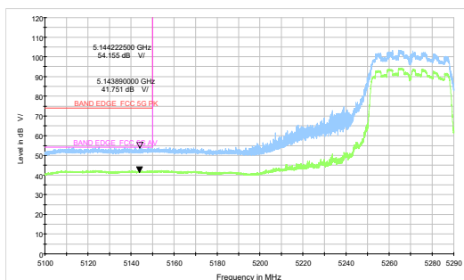
802.11ax HE40-Channel 54: Peak + Average
