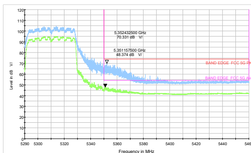
802.11ax HE40-Channel 62: Peak + Average
