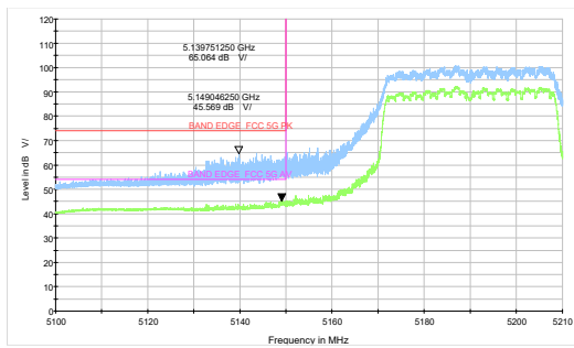
802.11ax HE40-Channel 38: Peak + Average
