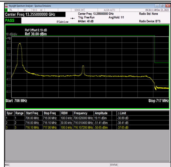
Band12_10MHz_16QAM_23130_1RB#0
