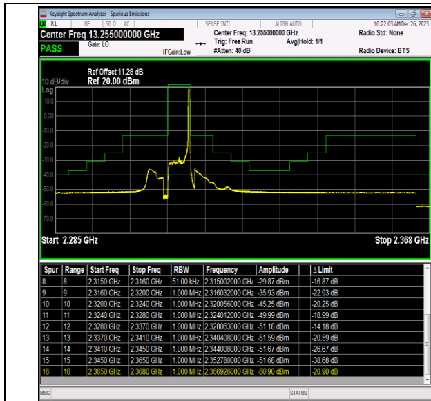
Band40_5MHz_QPSK_38775_1RB#24
