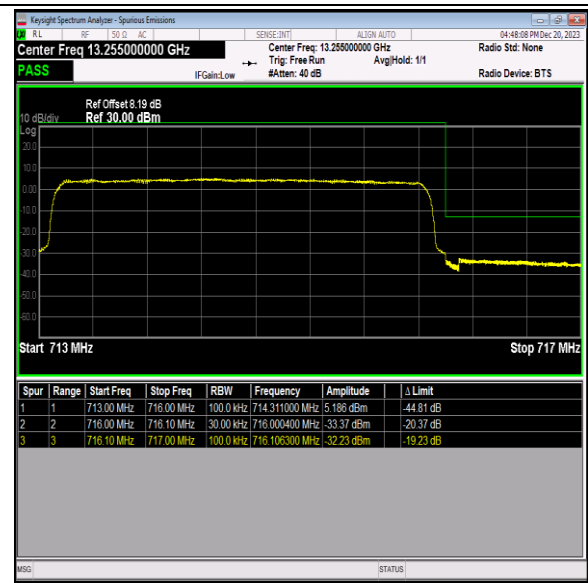
Band12_3MHz_16QAM_23165_15RB#0
