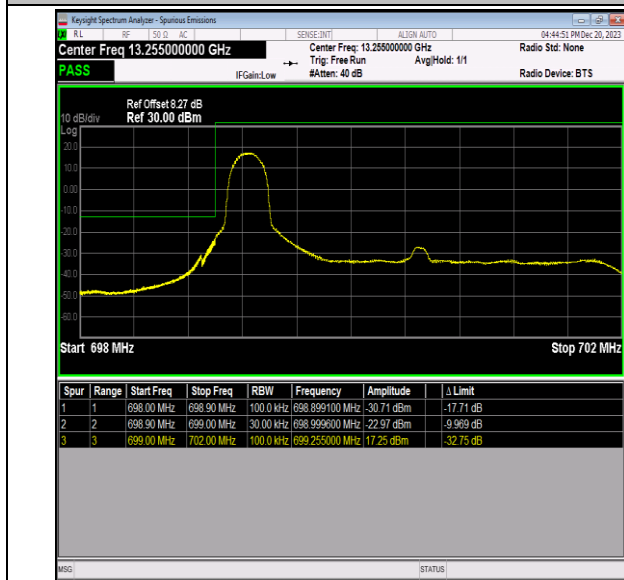
Band12_3MHz_64QAM_23025_1RB#0
