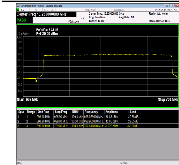
Band12_10MHz_16QAM_23060_50RB#0
