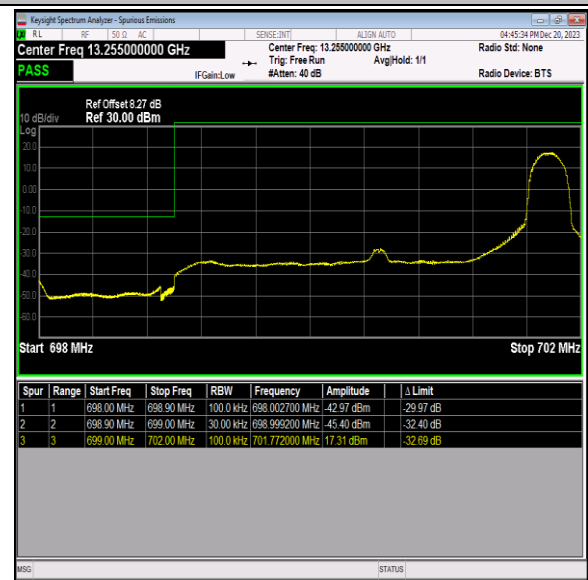
Band12_3MHz_64QAM_23025_1RB#14
