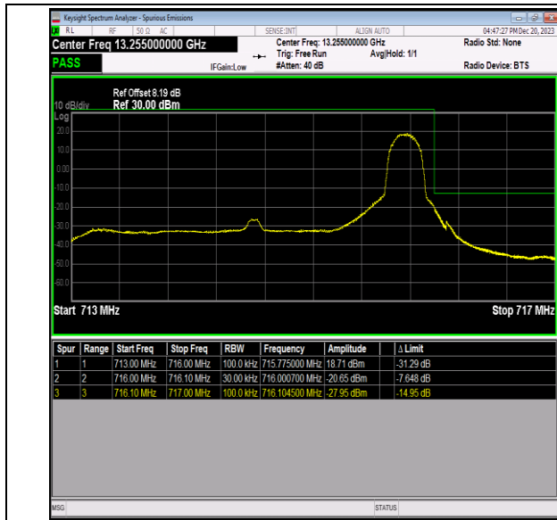
Band12_3MHz_16QAM_23165_1RB#14
