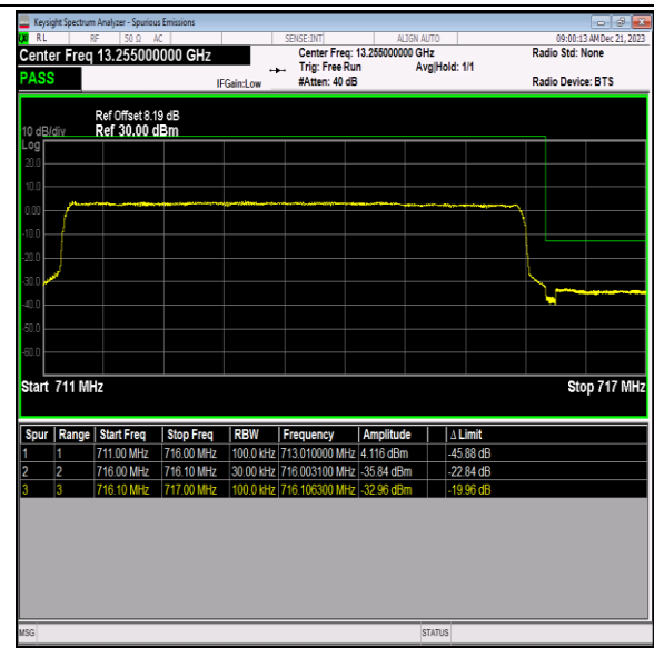
Band12_5MHz_QPSK_23155_25RB#0
