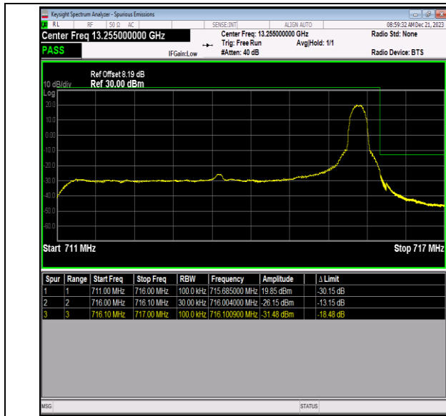
Band12_5MHz_QPSK_23155_1RB#24
