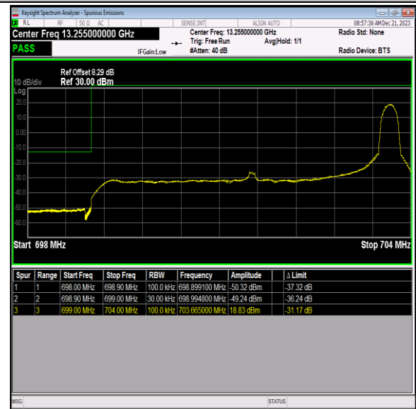
Band12_5MHz_16QAM_23035_1RB#24
