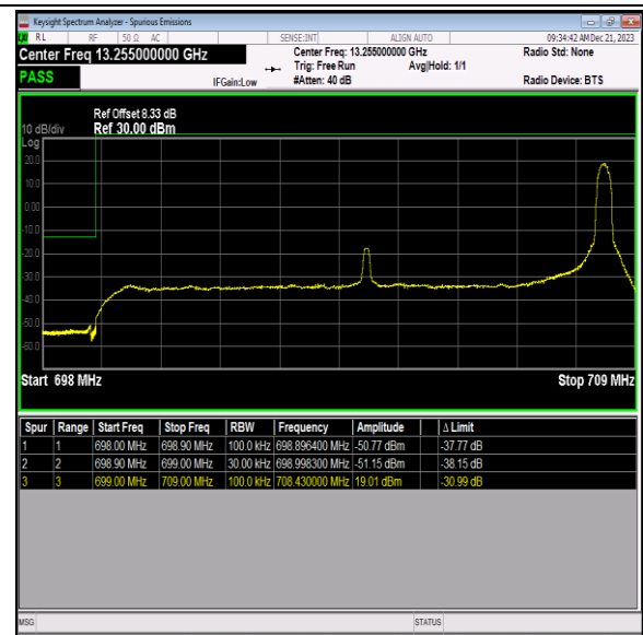
Band12_10MHz_16QAM_23060_1RB#49
