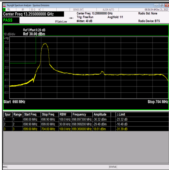
Band12_5MHz_16QAM_23035_1RB#0
