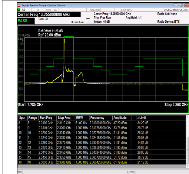
Band40_5MHz_16QAM_38725_1RB#0
