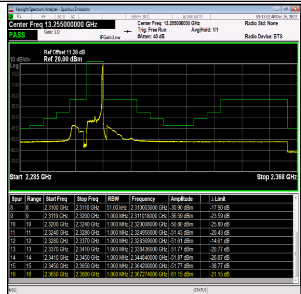
Band40_5MHz_16QAM_38725_1RB#24
