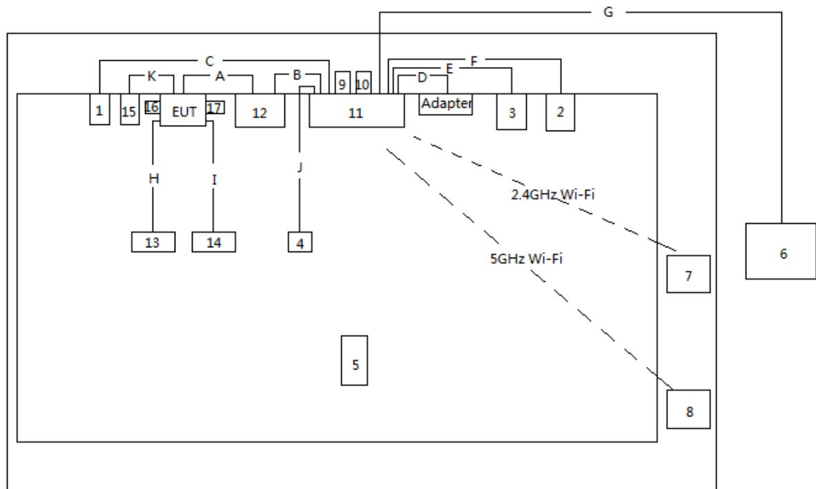
Connection Diagram(Mode 1)
