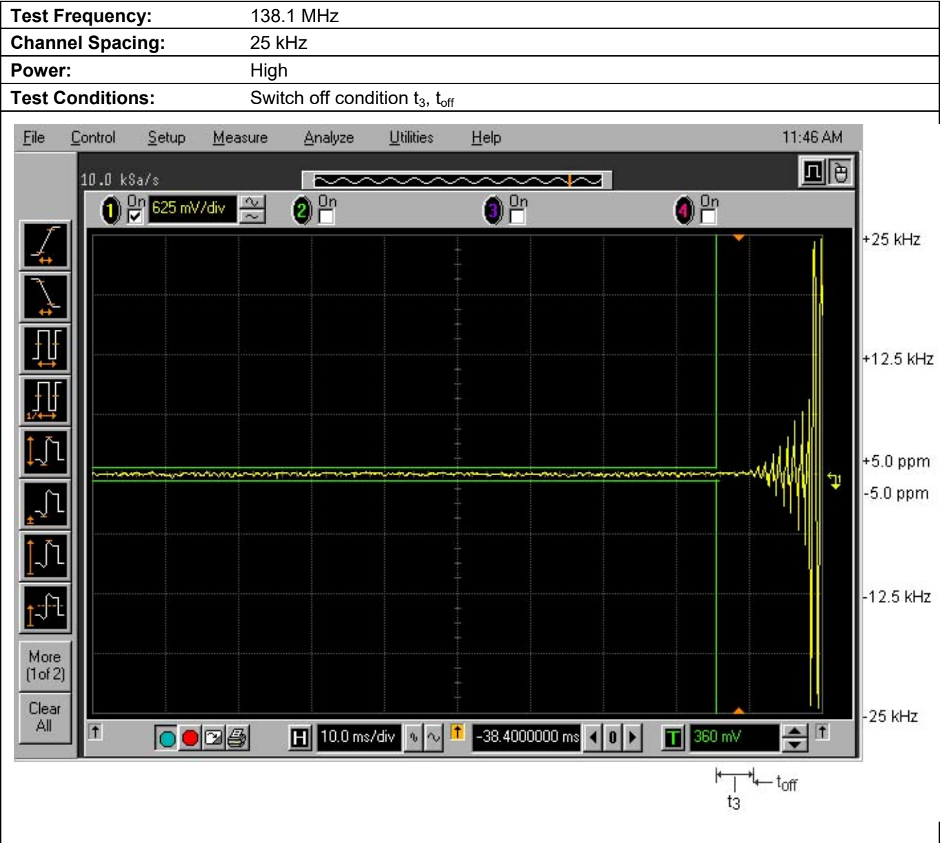
Plot 5.12.3.6. Transient Frequency Behavior for 25 kHz Channel Spacing
