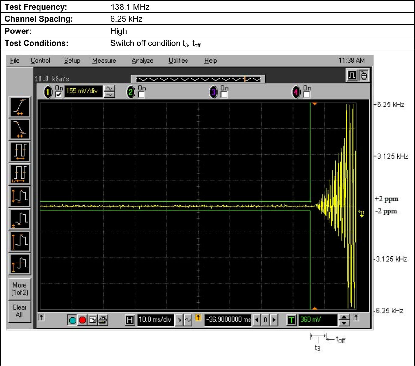
Plot 5.12.3.2. Transient Frequency Behavior for 6.25 kHz Channel Spacing
