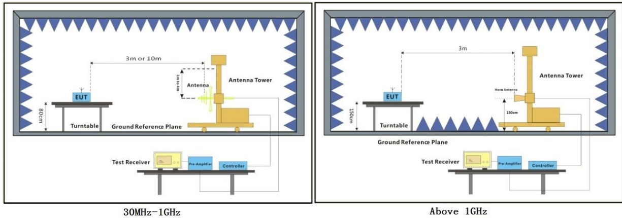
30MHz-1GHz
