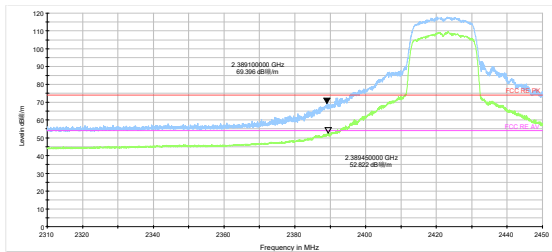
802.11n HT20-Channel 3 Peak+ Average
