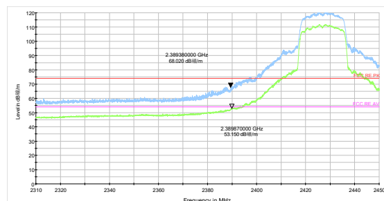
802.11n HT20-Channel 4 Peak+ Average
