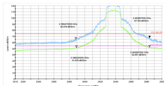
802.11n HT20-Channel 6 Peak+ Average
