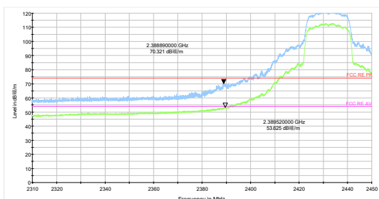
802.11n HT20-Channel 5 Peak+ Average
