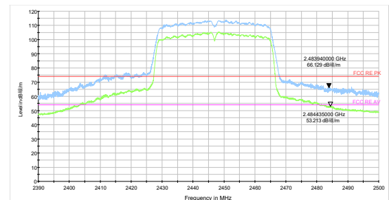
802.11n HT40-Channel 8 Peak+ Average
