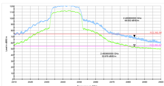
802.11n HT20-Channel 7 Peak+ Average
