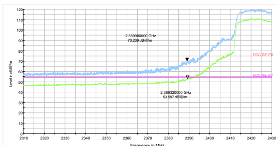
802.11n HT20-Channel 3 Peak+ Average
