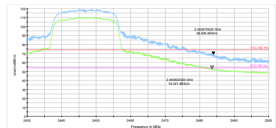
802.11n HT20-Channel 8 Peak+ Average
