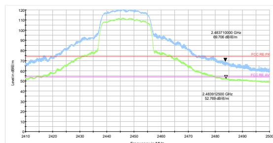
802.11n HT20-Channel 8 Peak+ Average
