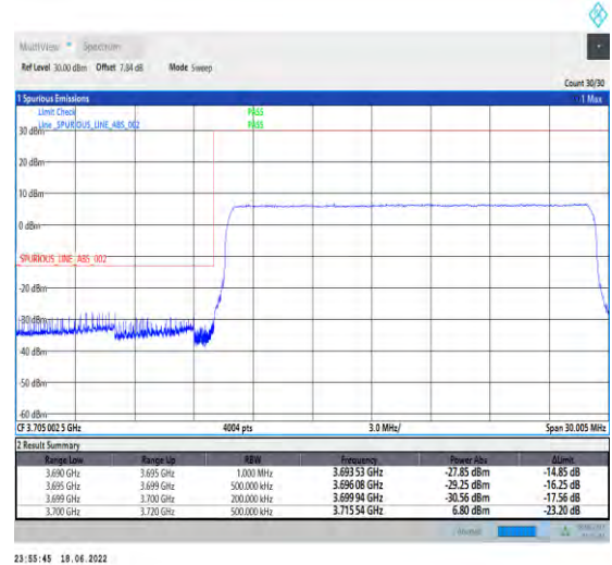
1-N77-3700-3980--30-20-L-6-CP-QPSK-Outer_Ful I-51@0-Ant1-PASS-see graph
