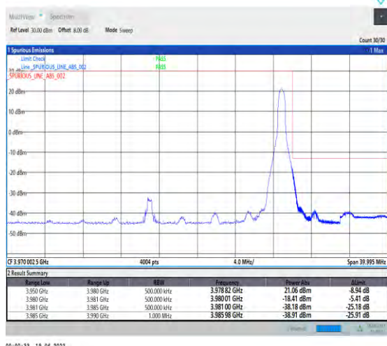
1-N77-3700-3980--30-30-H-2-DFT-PI2BPSK-Edge_1R B_Right-1@77-Ant1-PASS-see graph
