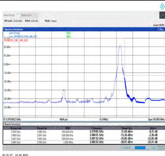
1-N77-3700-3980--30-30-H-5-CP-QPSK-Edge_1RB_R ight-1@77-Ant1-PASS-see graph
