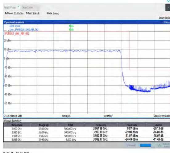
1-N77-3700-3980--30-30-H-3-DFT-PI2BPSK-Outer _Full-75@0-Ant1-PASS-see graph
