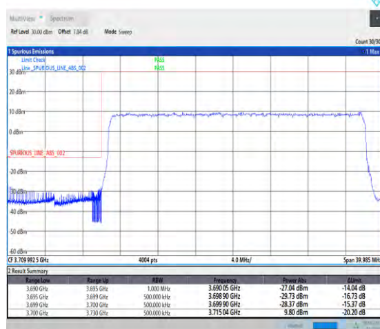
1-N77-3700-3980--30-30-L-3-DFT-PI2BPSK-Outer _Full-75@0-Ant1-PASS-see graph
