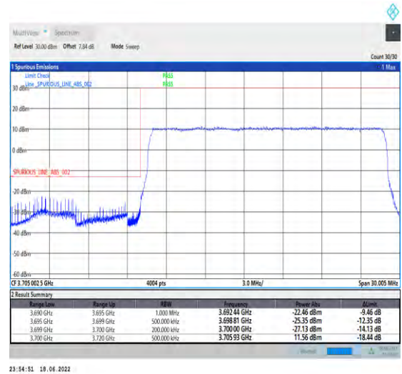
1-N77-3700-3980--30-20-L-3-DFT-PI2BPSK-Outer _Full-50@0-Ant1-PASS-see graph
