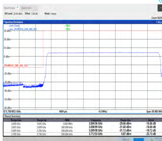
1-N77-3700-3980--30-30-L-6-CP-QPSK-Outer_Ful l-78@0-Ant1-PASS-see graph
