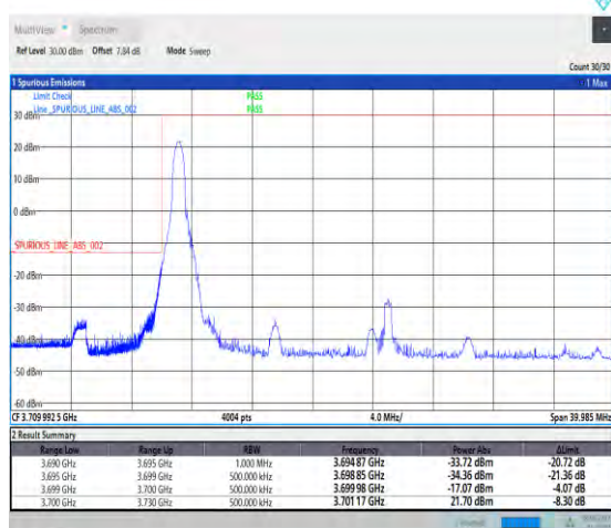
1-N77-3700-3980--30-30-L-4-CP-QPSK-Edge_1RB_L eft-1@0-Ant1-PASS-see graph
