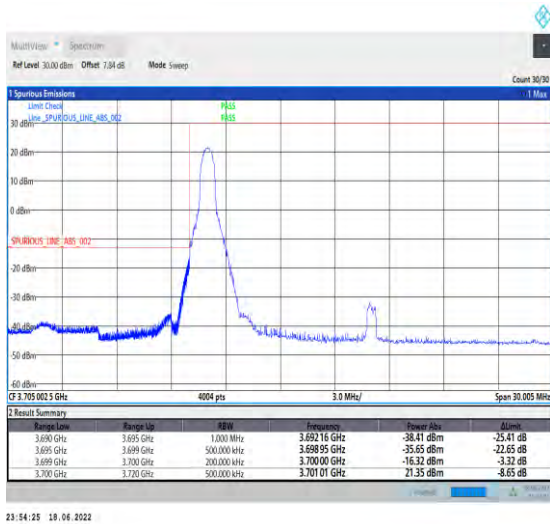
1-N77-3700-3980--30-20-L-1-DFT-PI2BPSK-Edge_1R B_Left-1@0-Ant1-PASS-see graph
