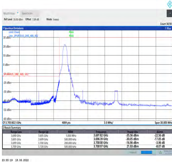
1-N77-3700-3980--30-20-L-4-CP-QPSK-Edge_1RB_L eft-1@0-Ant1-PASS-see graph
