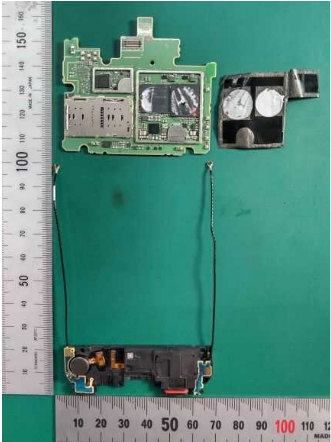
Main PCB, Front 2
