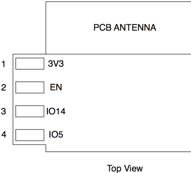
Figure 2-1. ESP-WROOM-5C Pin Layout (Top View)
