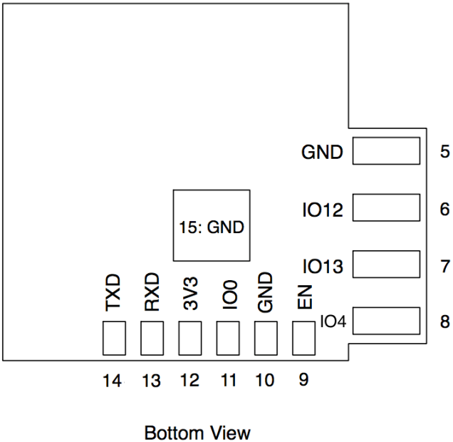
Figure 2-2. ESP-WROOM-5C Pin Layout (Bottom View)
