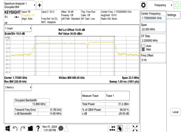
Band66B_10MHz+5MHz_256QAM_RB50-0+RB25-0_CH132397+CH132469
