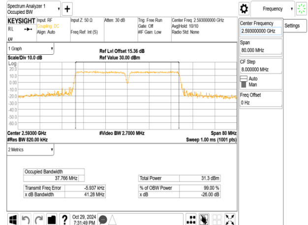
Band41_20MHz+20MHz_256QAM_RB100-0+RB100-0_CH40521+CH40719
