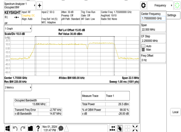
Band66B_5MHz+15MHz_QPSK_RB25-0+RB75-0_CH132353+CH132446
