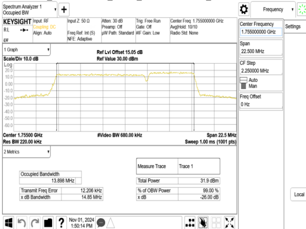
Band66B_10MHz+5MHz_16QAM_RB50-0+RB25-0_CH132397+CH132469
