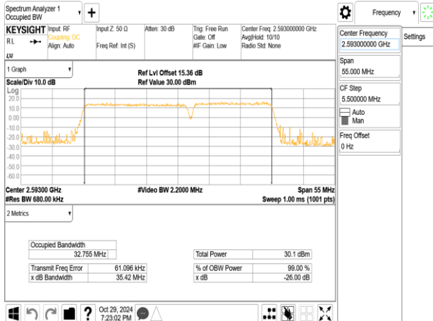
Band41_20MHz+20MHz_QPSK_RB100-0+RB100-0_CH40521+CH40719
