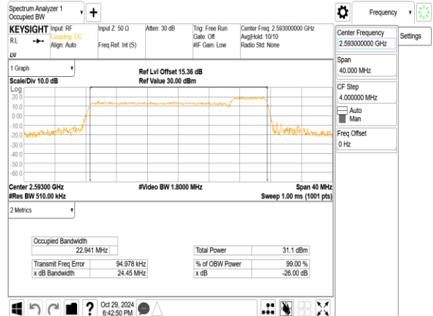
Band41_20MHz+5MHz_256QAM_RB100-0+RB25-0_CH40595+CH40712
