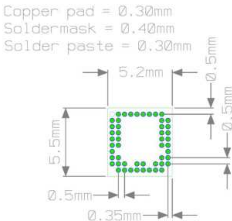
Figure 9.1. A121 footprint.
