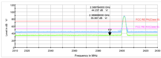
Bluetooth LE Channel 0 Peak &amp; Average
