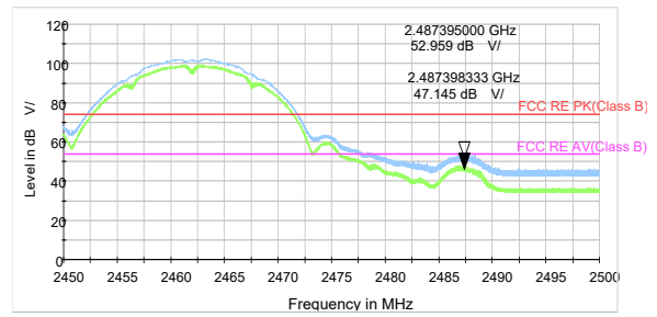
802.11b-Channel 11 Peak &amp; Average
