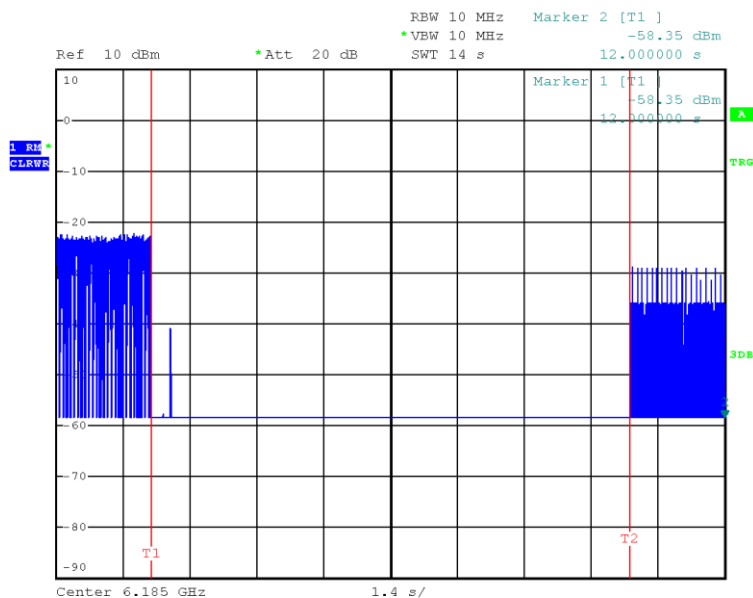
Frequency (MHz): 6185 MHz (Threshold Level: -60dBm)
