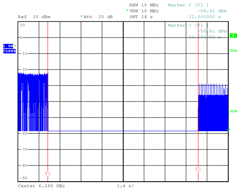
Frequency (MHz): 6185 MHz (Threshold Level: -59dBm)
