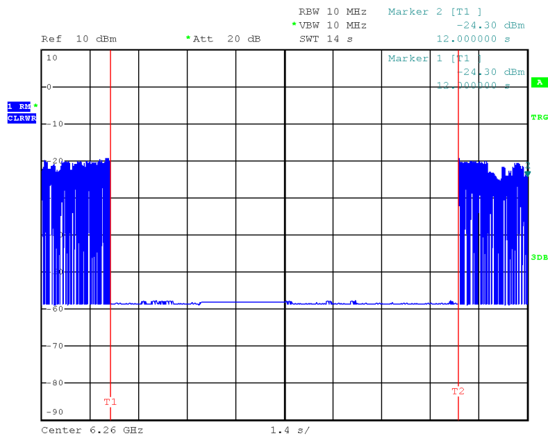
Test CH 47 ; Incumbent signal 6260 MHz
