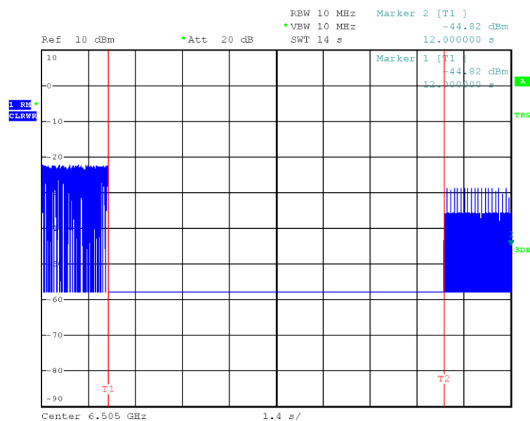
Test CH 111 ; Incumbent signal 6430 MHz
