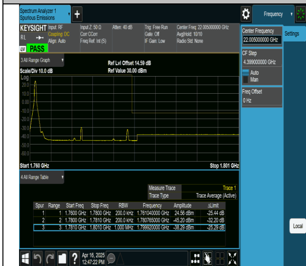
66-66-15MHz-5MHz-QPSK@QPSK-QPSK@QPSK-132549- 132642-1RB#0@0RB#0-0RB#0@0RB#0-PASS
