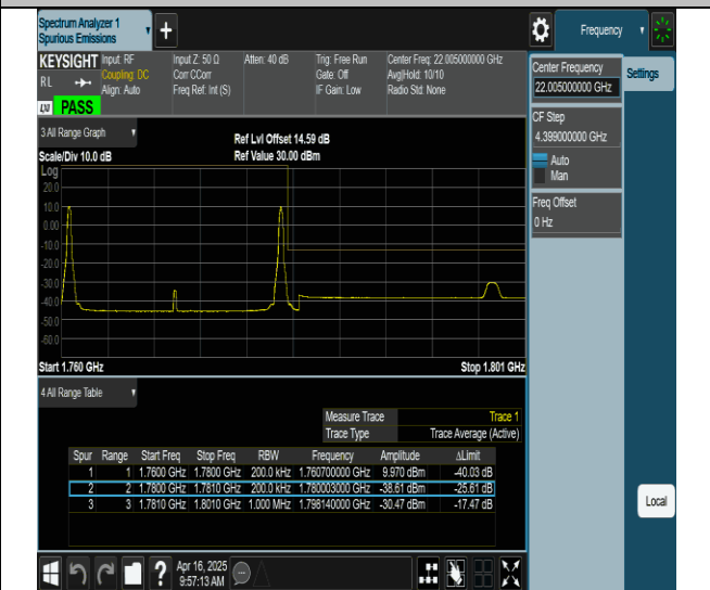
66-66-10MHz-10MHz-QPSK@QPSK-QPSK@QPSK-132523-132622-1RB#0@0RB#0-1RB#49@0RB#0-PASS
