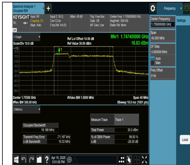
66-66-5MHz-15MHz-QPSK-QPSK-132353-132446-25RB#0- 75RB#0-PASS
