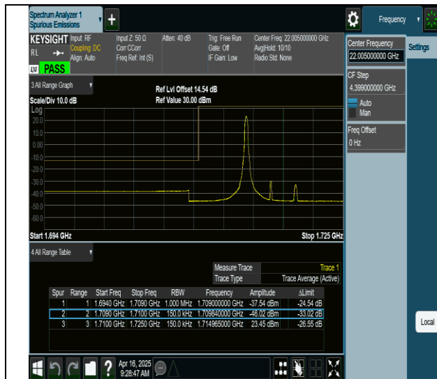
66-66-5MHz-10MHz-QPSK@QPSK-QPSK@QPSK-132000-132072-1RB#24@0RB#0-0RB#0@0RB#0-PASS
