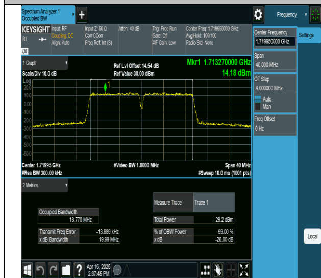
66-66-10MHz-10MHz-64QAM-64QAM-132022-132121-50RB#0-50RB#0-PASS
