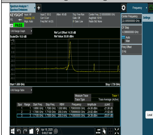
66-66-10MHz-10MHz-QPSK@QPSK-QPSK@QPSK-132022- 132121-1RB#0@0RB#0-0RB#0@0RB#0-PASS
