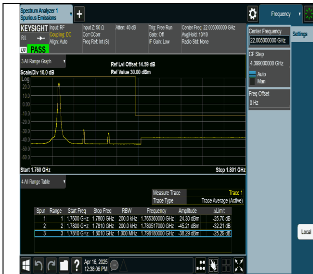
66-66-5MHz-15MHz-QPSK@QPSK-QPSK@QPSK-132504-132597-1RB#24@0RB#0-0RB#0-PASS
