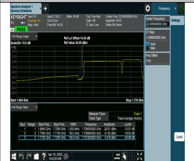
66-66-10MHz-5MHz-QPSK@QPSK-QPSK@QPSK-132022-132094-50RB#0@0RB#0-25RB#0@0RB#0-PASS
