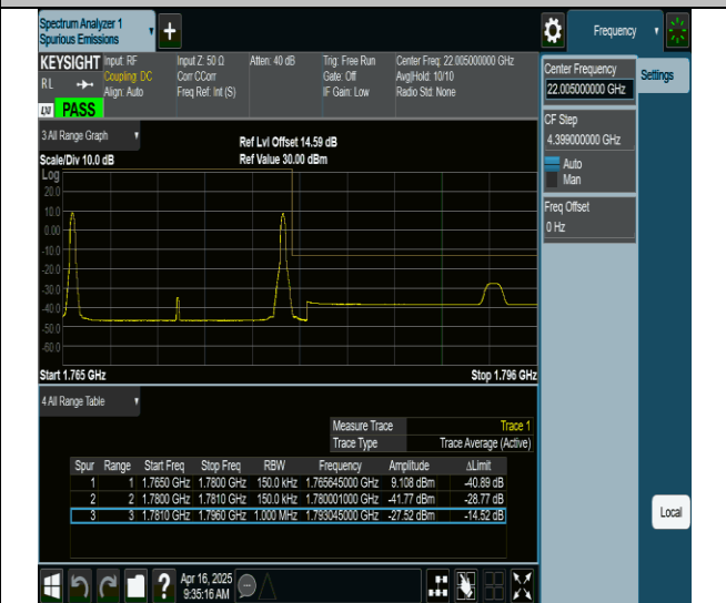
66-66-5MHz-10MHz-QPSK@QPSK-QPSK@QPSK-132550-132622-1RB#0@0RB#0-1RB#49@0RB#0-PASS
