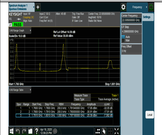
66-66-5MHz-15MHz-QPSK@QPSK-QPSK@QPSK-132504-132597-1RB#0@0RB#0-1RB#74@0RB#0-PASS
