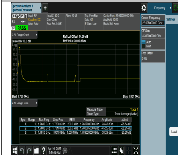
66-66-10MHz-10MHz-QPSK@QPSK-QPSK@QPSK-132523-132622-1RB#0@0RB#0-0RB#0@0RB#0-PASS
