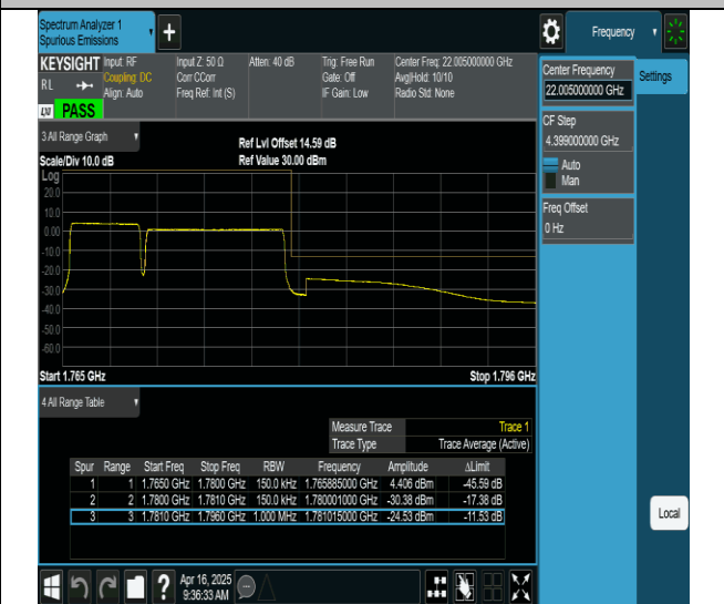
66-66-5MHz-10MHz-QPSK@QPSK-QPSK@QPSK-132550-132622-25RB#0@0RB#0-50RB#0@0RB#0-PASS
