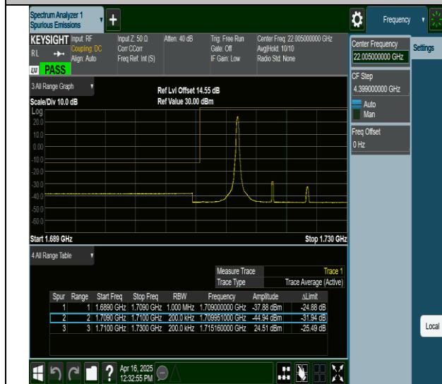
66-66-5MHz-15MHz-QPSK@QPSK-QPSK@QPSK-132002-132095-1RB#24@0RB#0-0RB#0@0RB#0-PASS
