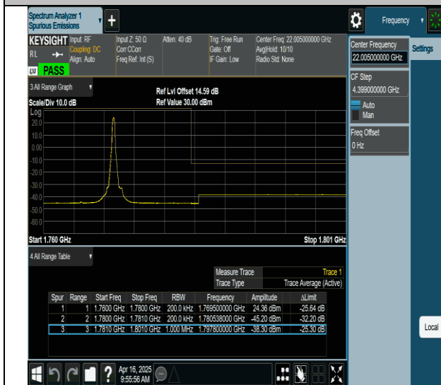
66-66-10MHz-10MHz-QPSK@QPSK-QPSK@QPSK-132523-132622-1RB#49@0RB#0-0RB#0@0RB#0-PASS
