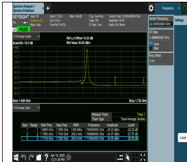
66-66-5MHz-15MHz-QPSK@QPSK-QPSK@QPSK-132002-132095-1RB#0@0RB#0-0RB#0@0RB#0-PASS
