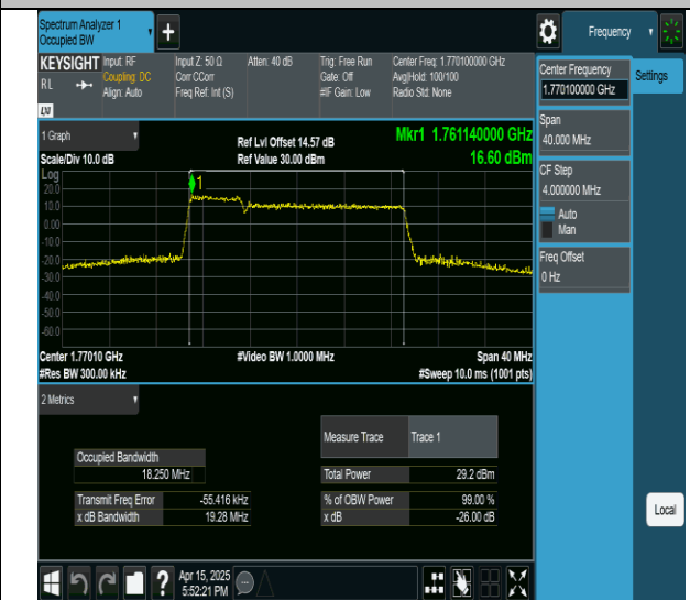
66-66-5MHz-15MHz-16QAM-16QAM-132504-132597-25RB#0- 75RB#0-PASS
