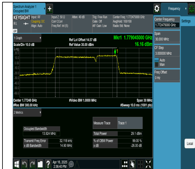
66-66-10MHz-5MHz-64QAM-64QAM-132572-132644-50RB#0-25RB#0-PASS
