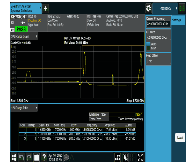
66-66-5MHz-15MHz-QPSK@QPSK-QPSK@QPSK-132002-132095-1RB#0@0RB#0-1RB#74@0RB#0-PASS
