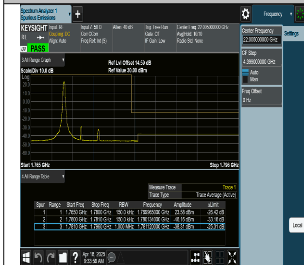
66-66-5MHz-10MHz-QPSK@QPSK-QPSK@QPSK-132550-132622-1RB#24@0RB#0-0RB#0@0RB#0-PASS
