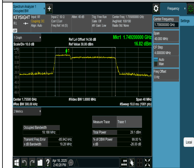
66-66-5MHz-15MHz-64QAM-64QAM-132353-132446-25RB#0- 75RB#0-PASS
