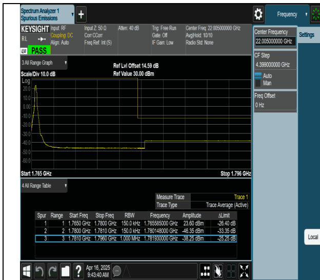
66-66-10MHz-5MHz-QPSK@QPSK-QPSK@QPSK-132572- 132644-1RB#0@0RB#0-0RB#0@0RB#0-PASS
