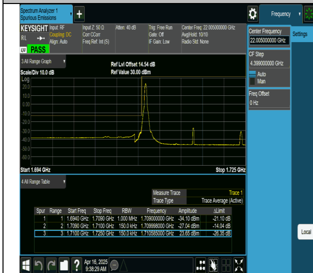
66-66-10MHz-5MHz-QPSK@QPSK-QPSK@QPSK-132022-132094-1RB#0@0RB#0-0RB#0@0RB#0-PASS
