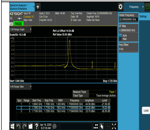
66-66-5MHz-10MHz-QPSK@QPSK-QPSK@QPSK-132000- 132072-1RB#0@0RB#0-0RB#0@0RB#0-PASS
