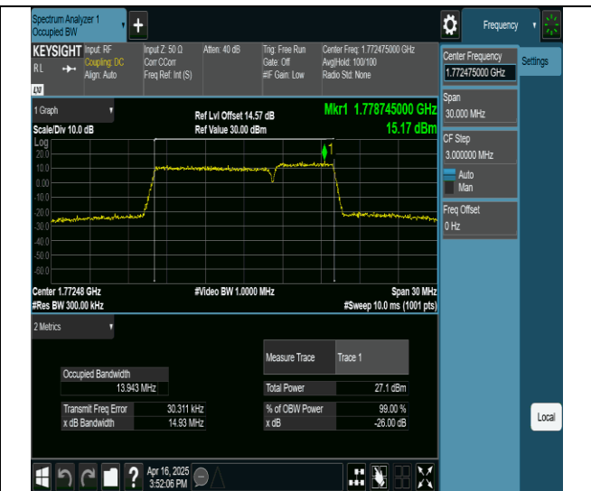
66-66-10MHz-5MHz-256QAM-256QAM-132572-132644-50RB#0-25RB#0-PASS
