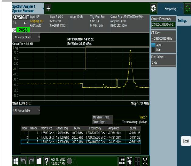
66-66-15MHz-5MHz-QPSK@QPSK-QPSK@QPSK-132047- 132140-1RB#74@0RB#0-0RB#0@0RB#0-PASS
