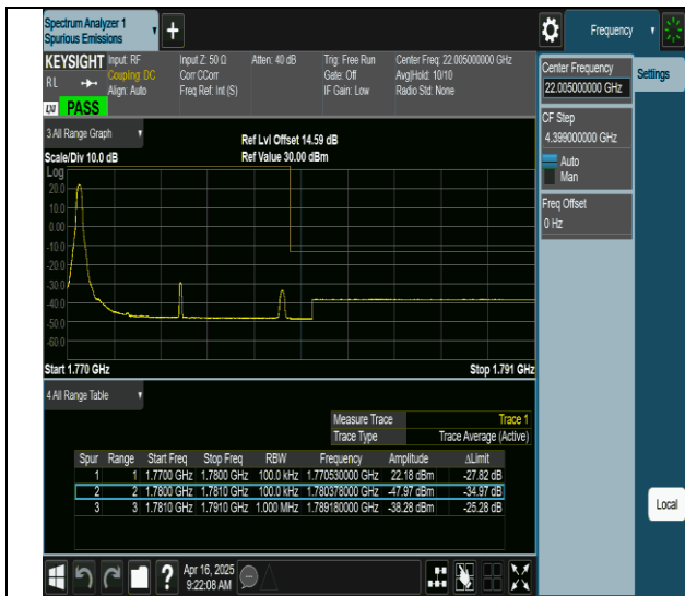
66-66-5MHz-5MHz-QPSK@QPSK-QPSK@QPSK-132599- 132647-1RB#0@0RB#0-0RB#0@0RB#0-PASS
