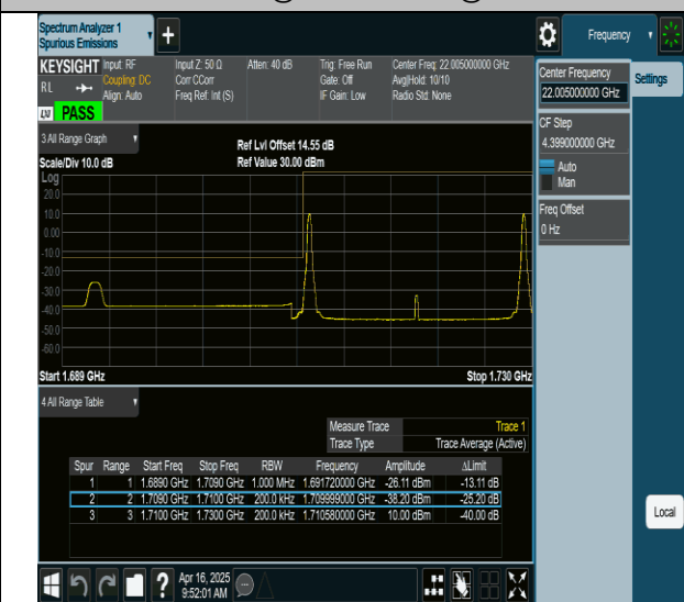
66-66-10MHz-10MHz-QPSK@QPSK-QPSK@QPSK-132022- 132121-1RB#0@0RB#0-1RB#49@0RB#0-PASS
