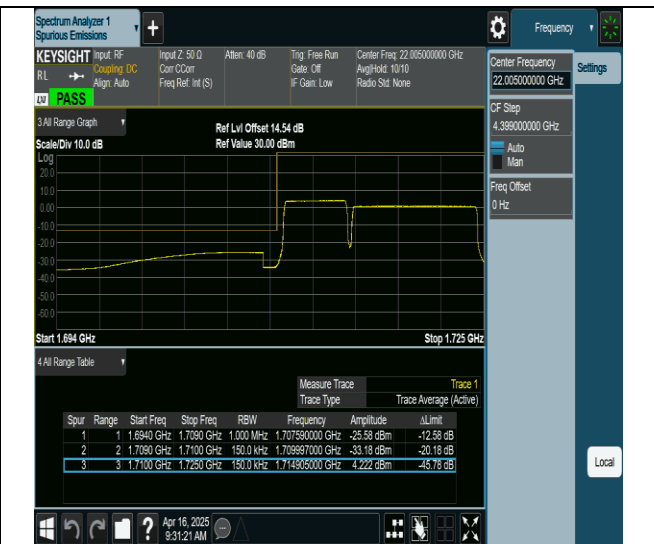
66-66-5MHz-10MHz-QPSK@QPSK-QPSK@QPSK-132000-132072-25RB#0@0RB#0-50RB#0@0RB#0-PASS
