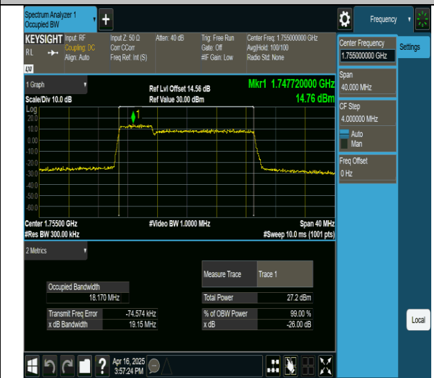
66-66-5MHz-15MHz-256QAM-256QAM-132353-132446-25RB#0- 75RB#0-PASS
