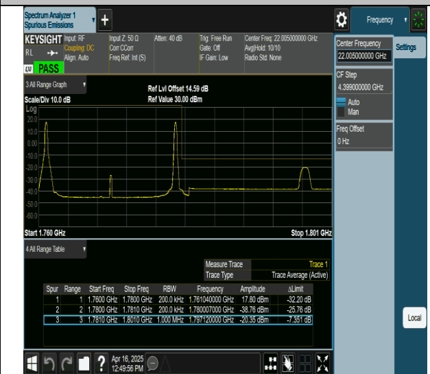
66-66-15MHz-5MHz-QPSK@QPSK-QPSK@QPSK-132549- 132642-1RB#0@0RB#0-1RB#24@0RB#0-PASS
