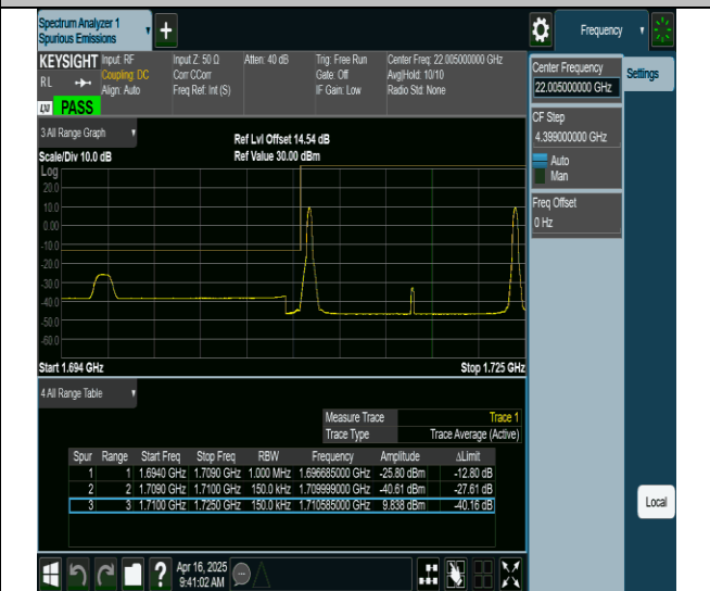
66-66-10MHz-5MHz-QPSK@QPSK-QPSK@QPSK-132022-132094-1RB#0@0RB#0-1RB#24@0RB#0-PASS
