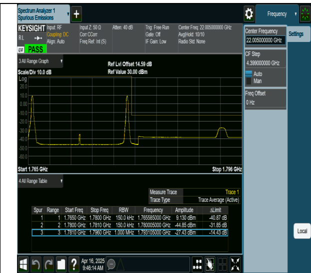
66-66-10MHz-5MHz-QPSK@QPSK-QPSK@QPSK-132572- 132644-1RB#0@0RB#0-1RB#24@0RB#0-PASS
