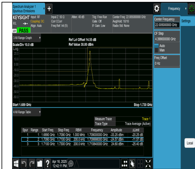
66-66-15MHz-5MHz-QPSK@QPSK-QPSK@QPSK-132047- 132140-1RB#0@0RB#0-0RB#0@0RB#0-PASS
