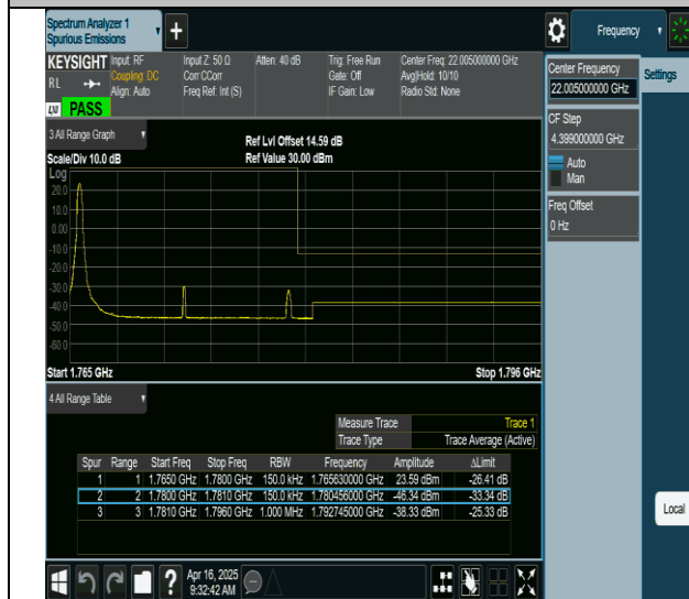
66-66-5MHz-10MHz-QPSK@QPSK-QPSK@QPSK-132550-132622-1RB#0@0RB#0-0RB#0@0RB#0-PASS
