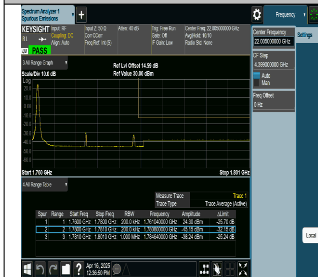
66-66-5MHz-15MHz-QPSK@QPSK-QPSK@QPSK-132504-132597-1RB#0@0RB#0-0RB#0@0RB#0-PASS
