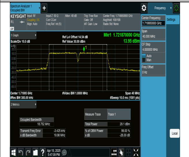
66-66-10MHz-10MHz-16QAM-16QAM-132022-132121-50RB#0-50RB#0-PASS
