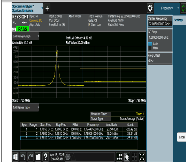
66-66-10MHz-5MHz-QPSK@QPSK-QPSK@QPSK-132572- 132644-1RB#49@0RB#0-0RB#0@0RB#0-PASS
