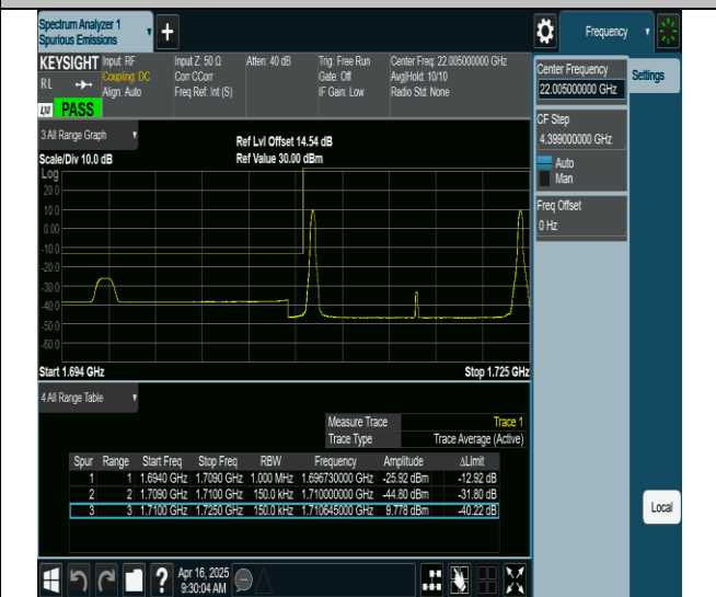
66-66-5MHz-10MHz-QPSK@QPSK-QPSK@QPSK-132000- 132072-1RB#0@0RB#0-1RB#49@0RB#0-PASS
