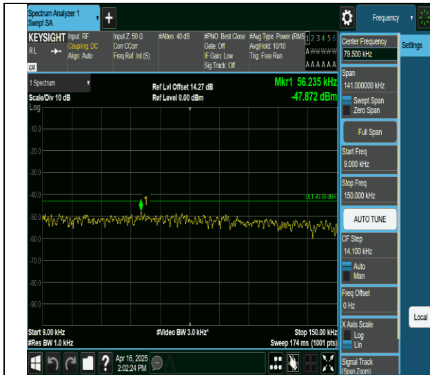
66-66-10MHz-10MHz-QPSK-QPSK-132523-132622-1RB#0- ORB#0-0.009~0.15MHz-PASS
