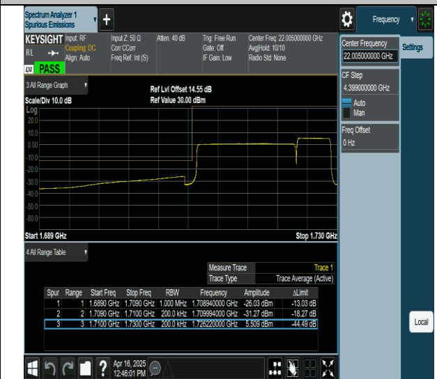
66-66-15MHz-5MHz-QPSK@QPSK-QPSK@QPSK-132047- 132140-75RB#0@0RB#0-25RB#0@0RB#0-PASS
