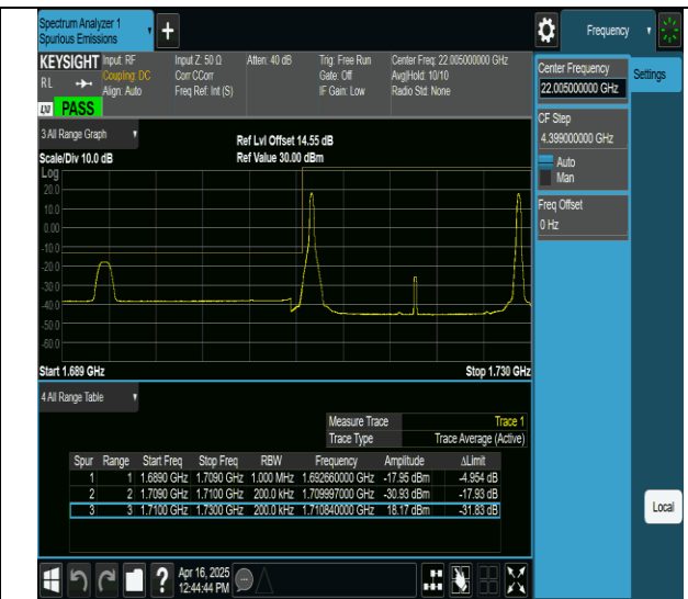
66-66-15MHz-5MHz-QPSK@QPSK-QPSK@QPSK-132047- 132140-1RB#0@0RB#0-1RB#24@0RB#0-PASS
