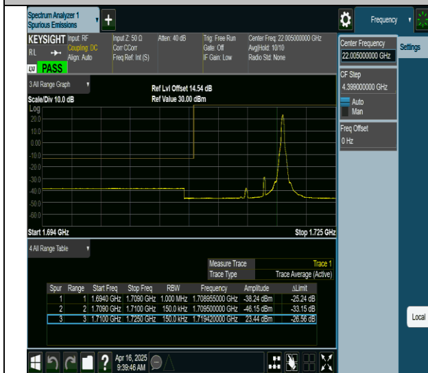
66-66-10MHz-5MHz-QPSK@QPSK-QPSK@QPSK-132022-132094-1RB#49@0RB#0-0RB#0@0RB#0-PASS
