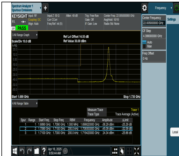
66-66-10MHz-10MHz-QPSK@QPSK-QPSK@QPSK-132022-132121-1RB#49@0RB#0-0RB#0@0RB#0-PASS
