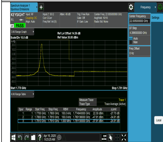
66-66-5MHz-5MHz-QPSK@QPSK-QPSK@QPSK-132599- 132647-1RB#24@0RB#0-0RB#0@0RB#0-PASS
