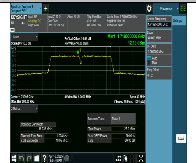
66-66-10MHz-10MHz-256QAM-256QAM-132022-132121-50RB#0-50RB#0-PASS
