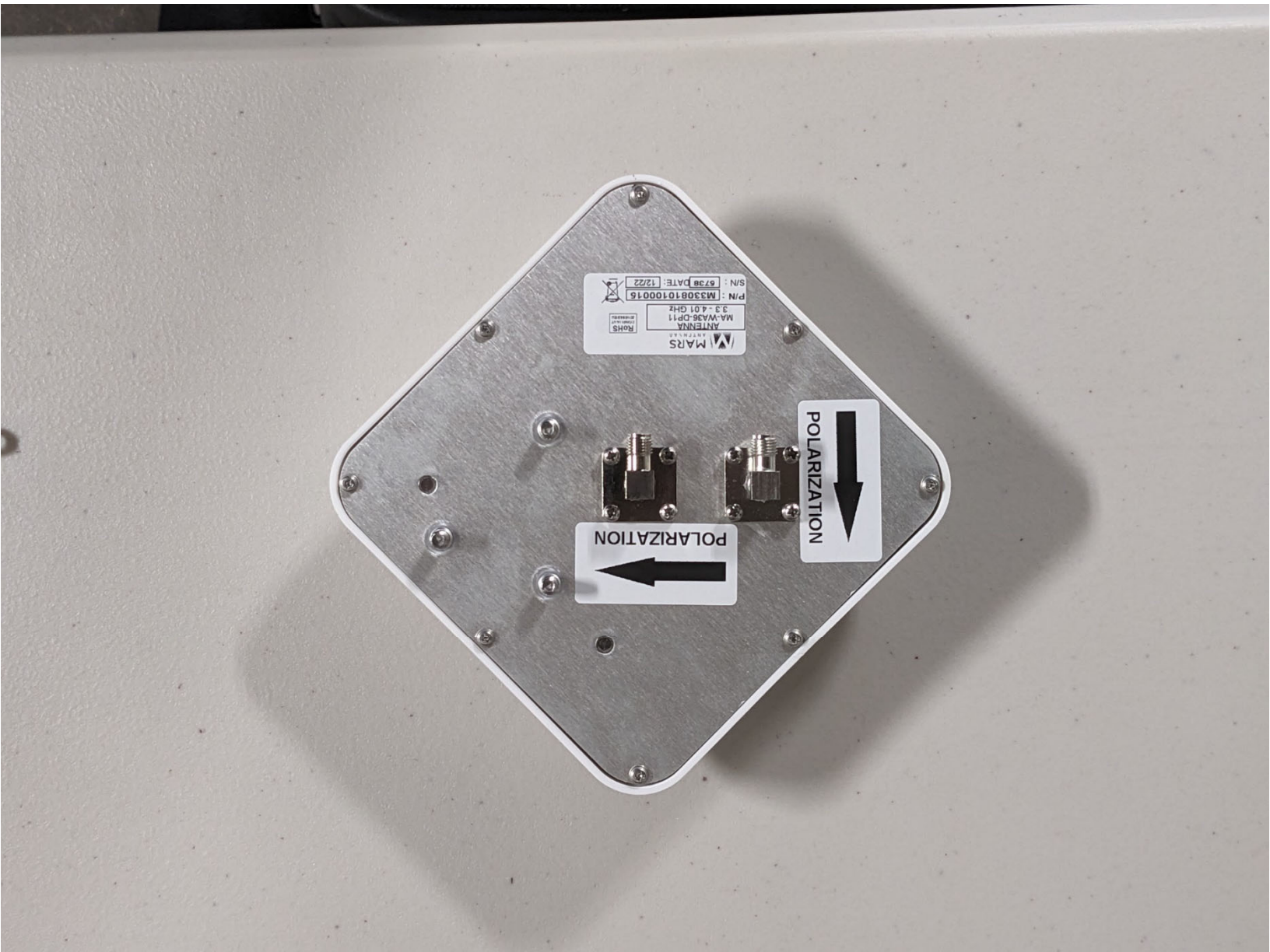
Rear View of Antenna Assembly
