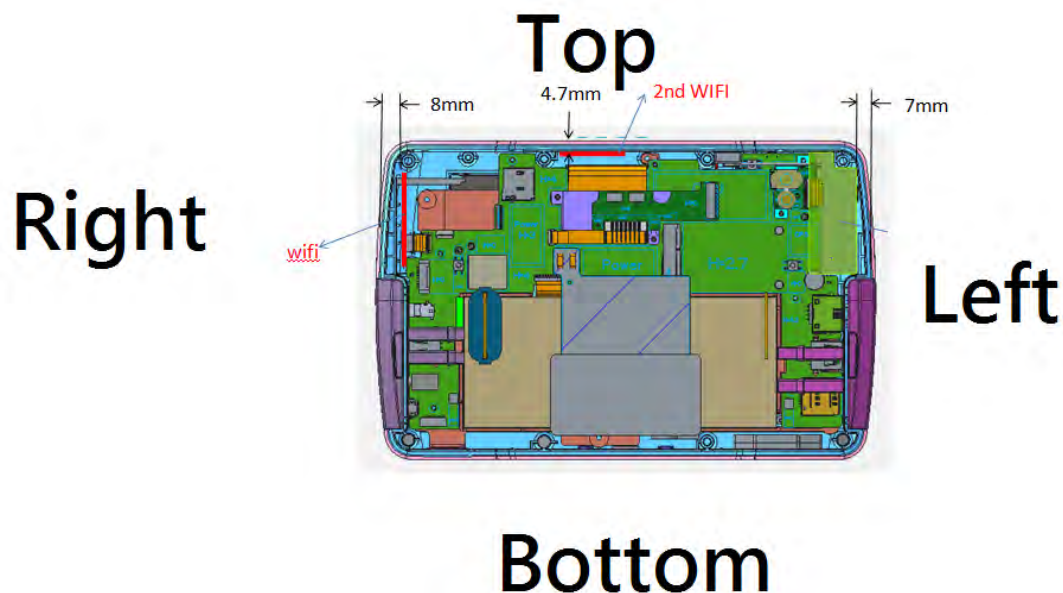
Fig.11 Antenna position of EUT (Back view)
