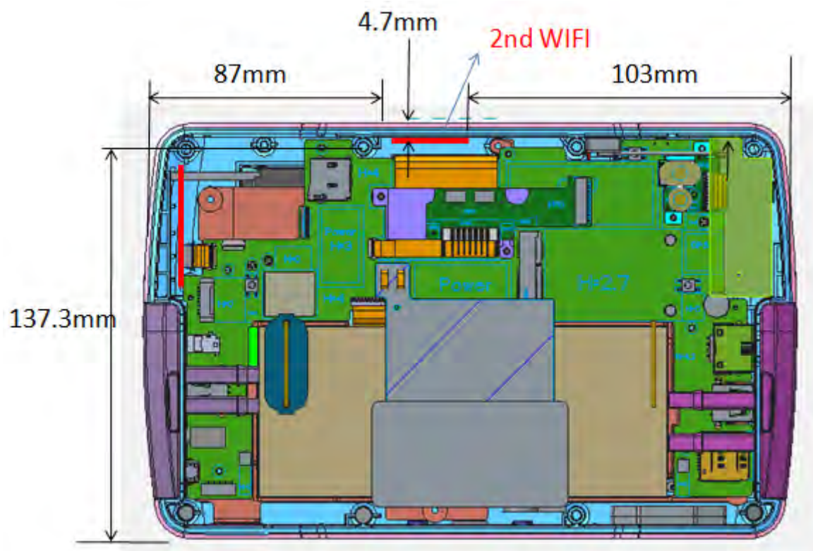
Fig.13 Antenna separation distance of EUT (WLAN Aux antenna)
