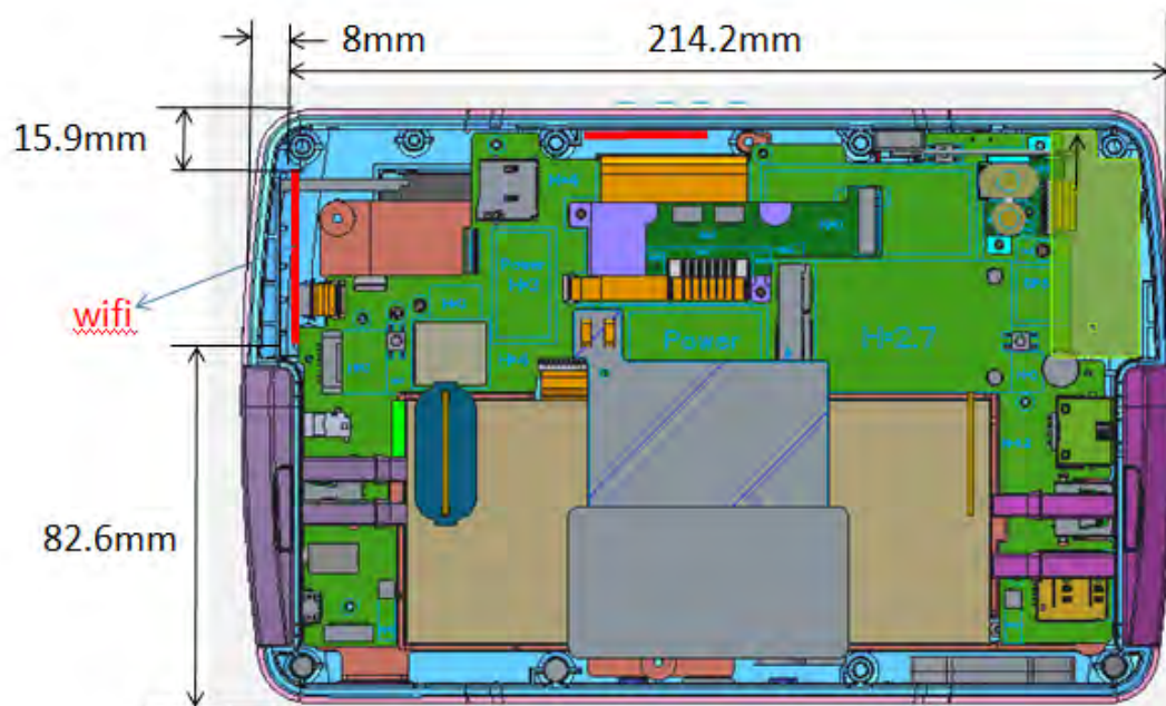
Fig.12 Antenna separation distance of EUT (WLAN Main/BT antenna)
