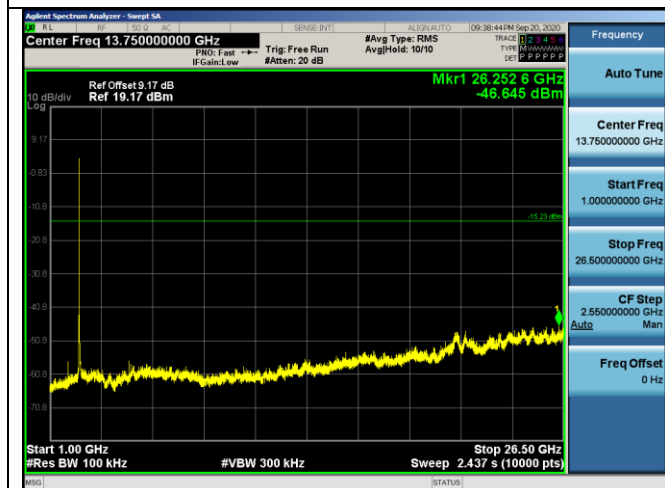
802.11b on Channel 09
