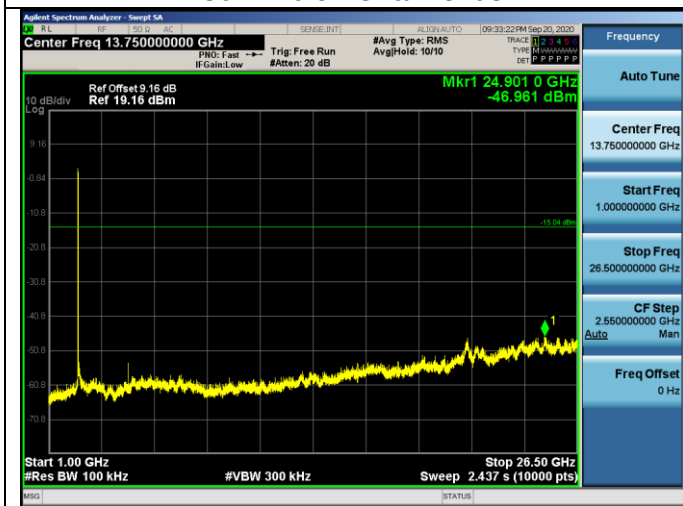
802.11b on Channel 03
