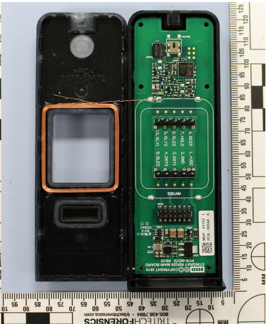
Model 20 (terminal version) case open rear view
