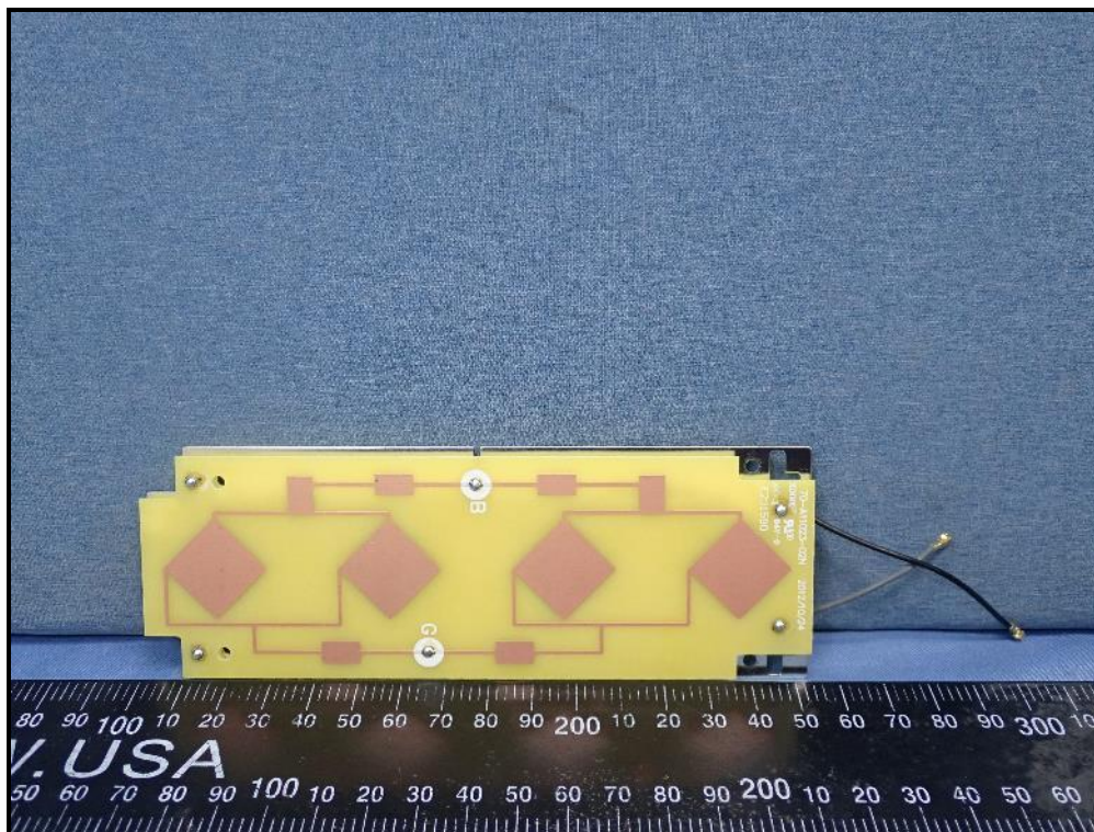
5G0+5G1 Antenna
