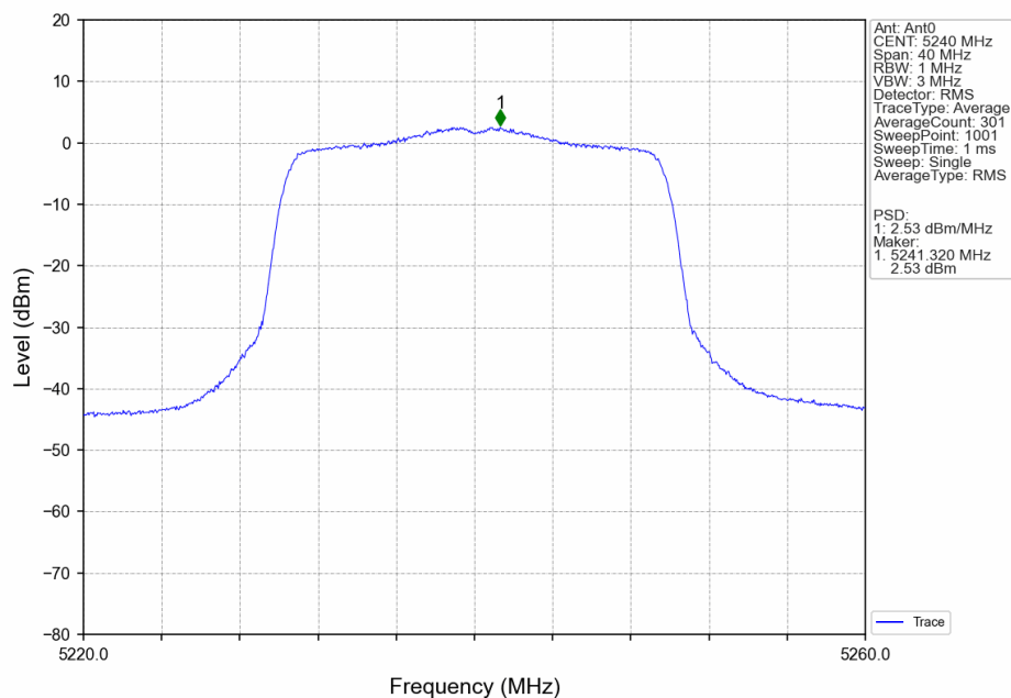
802.11ax(HEW20)_HCH_5240MHz_SU_ / _Ant0_NTNV
