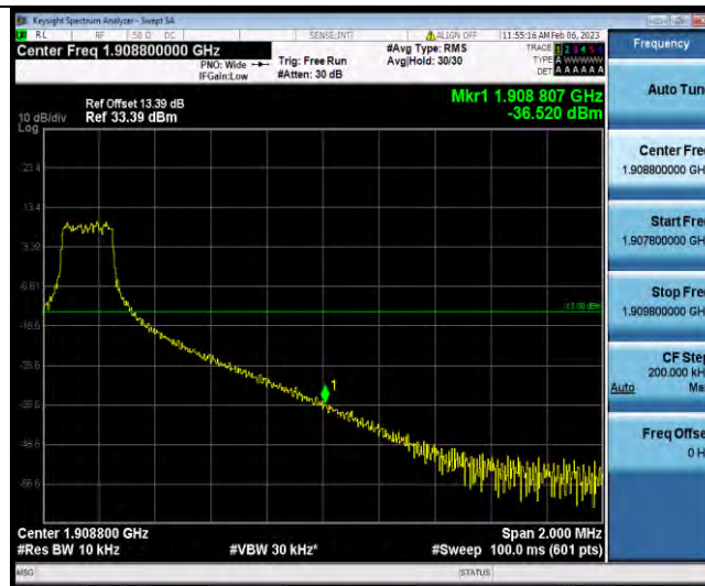
Band2-15MHz-64QAM-19125-75RB#0
