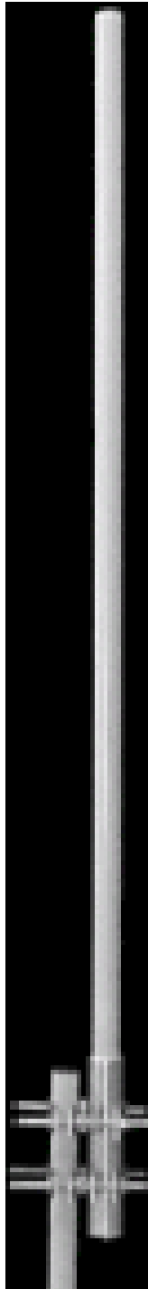
Photograph No.5 Omni-directional 360°/12 dBi antenna General view
