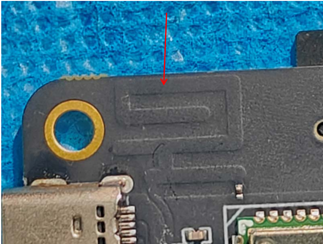
PCB Antenna
