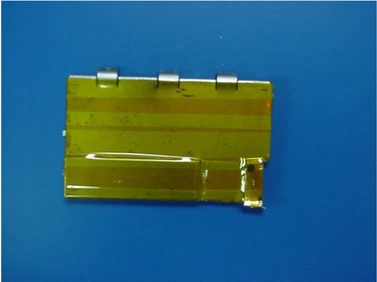
PHOTOGRAPH 13: TOP VIEW OF THE COVER FOR THE RF PORTION
