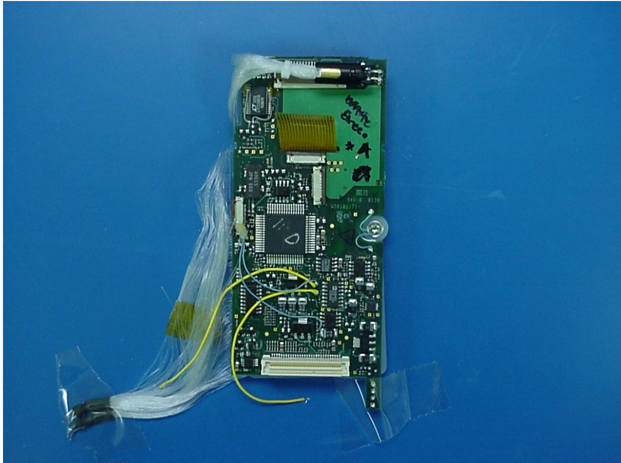
PHOTOGRAPH 16: TOP VIEW OF THE LOGIC BOARD
