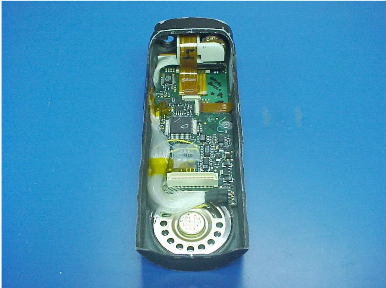
PHOTOGRAPH 10: SIDE VIEW OF THE RADIO WITHOUT THE RF PORTION
