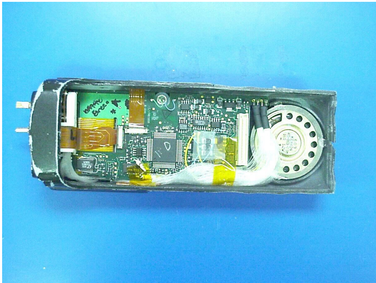
PHOTOGRAPH 9: INSIDE VIEW OF THE RADIO WITHOUT THE RF PORTION
