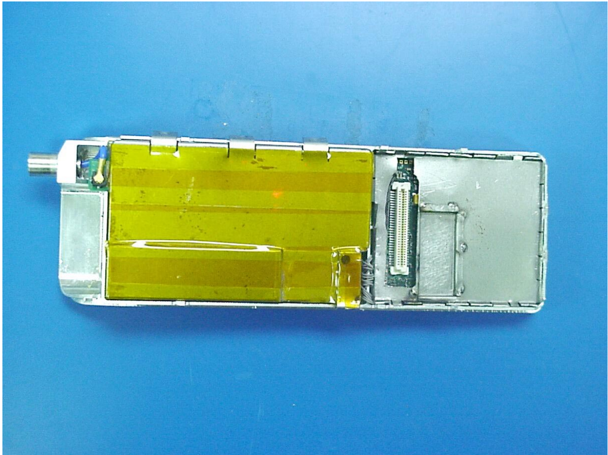
PHOTOGRAPH 11: RADIO RF AND LOGIC BOARDS WITH SHIELDS
