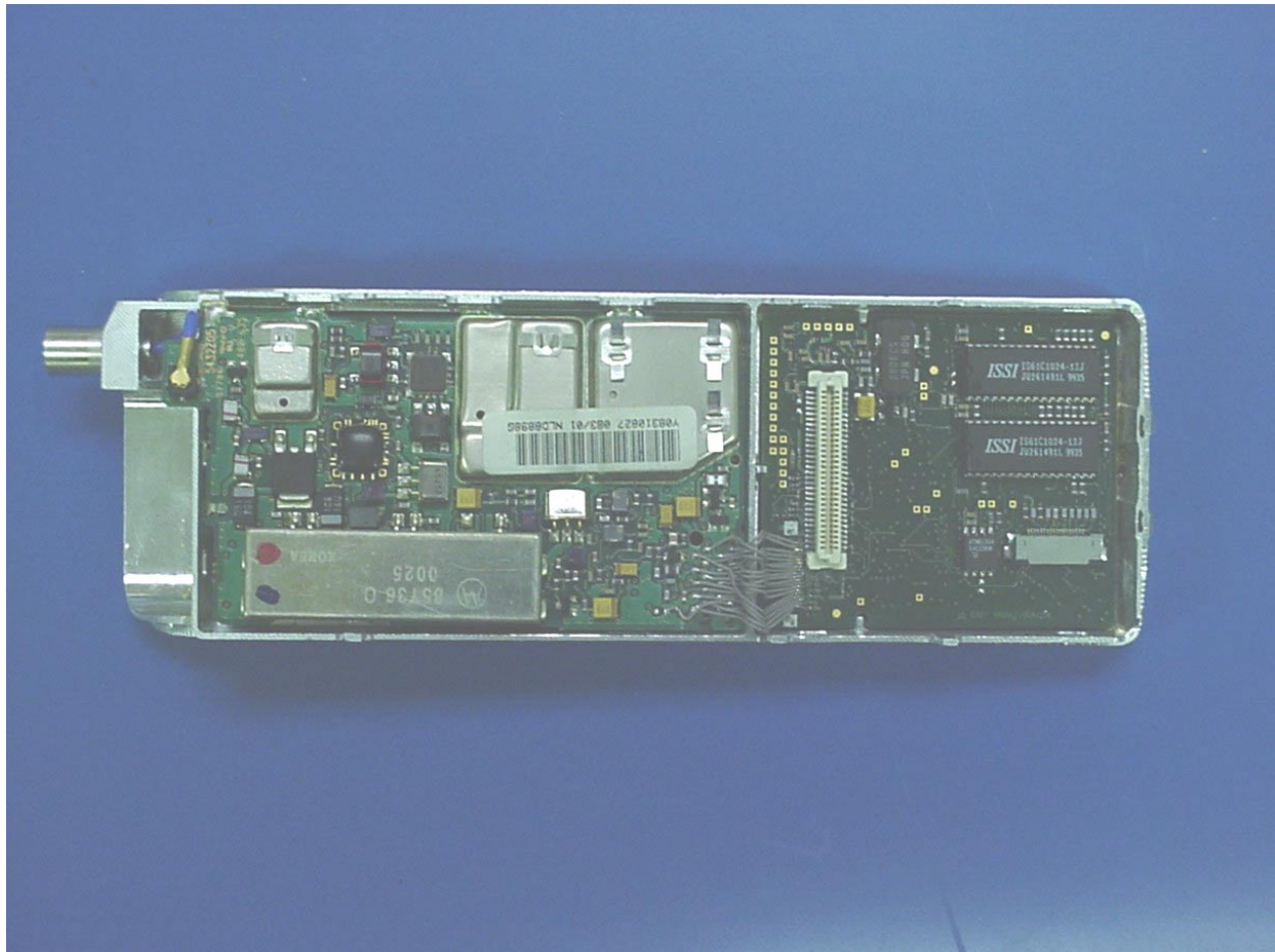
PHOTOGRAPH 15: RF AND LOGIC PART WITHOUT SHIELDS
