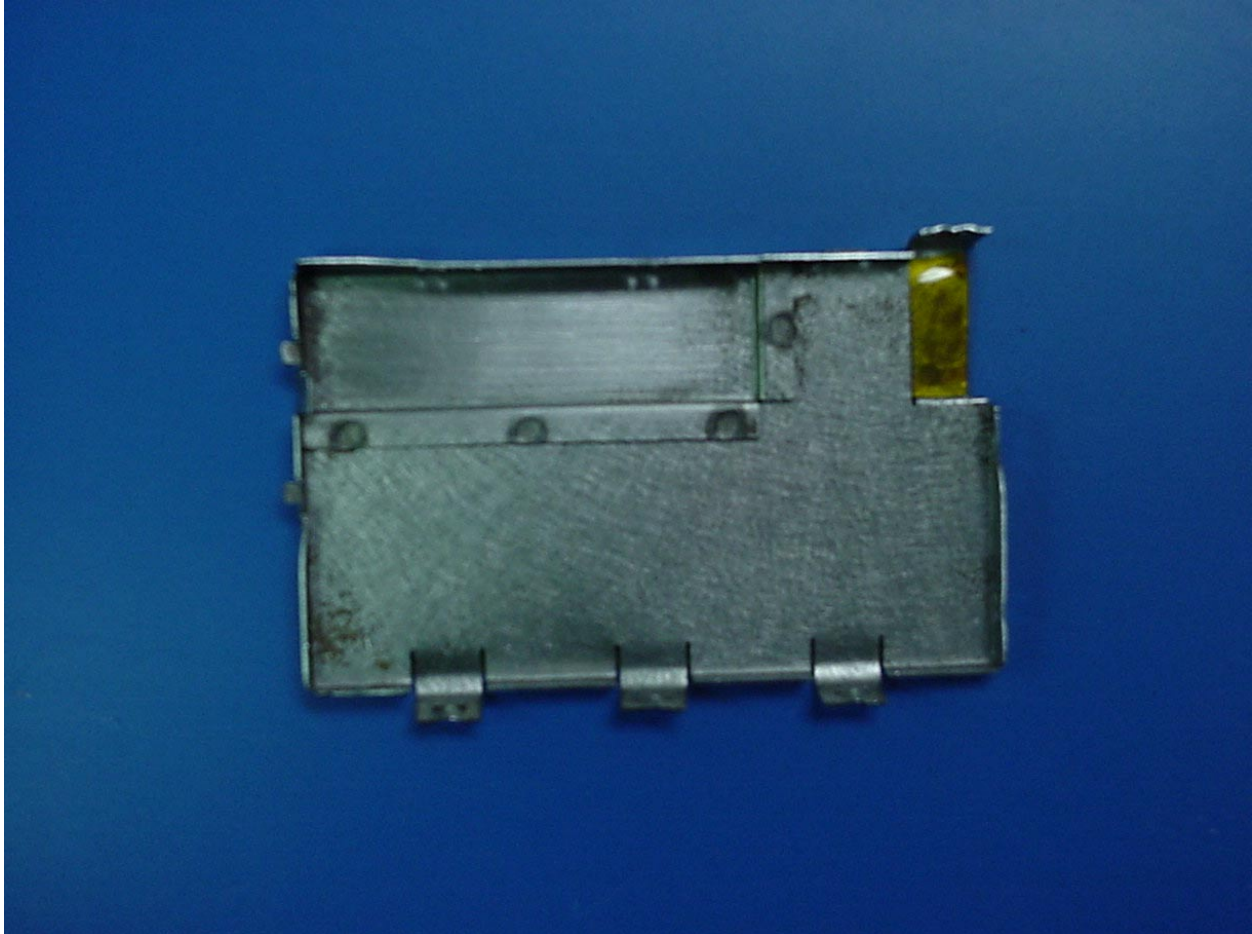
PHOTOGRAPH 14: BOTTOM VIEW OF THE COVER FOR THE RF PORTION
