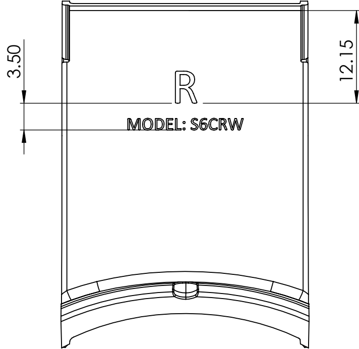
ARMATURE SLIDER COVER RIGHT RETAIL - TIER 1 P/N: 16H02-115R
