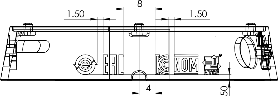
EAR CUP RING RIGHT - TIER 3 P/N: 16H02-102R
