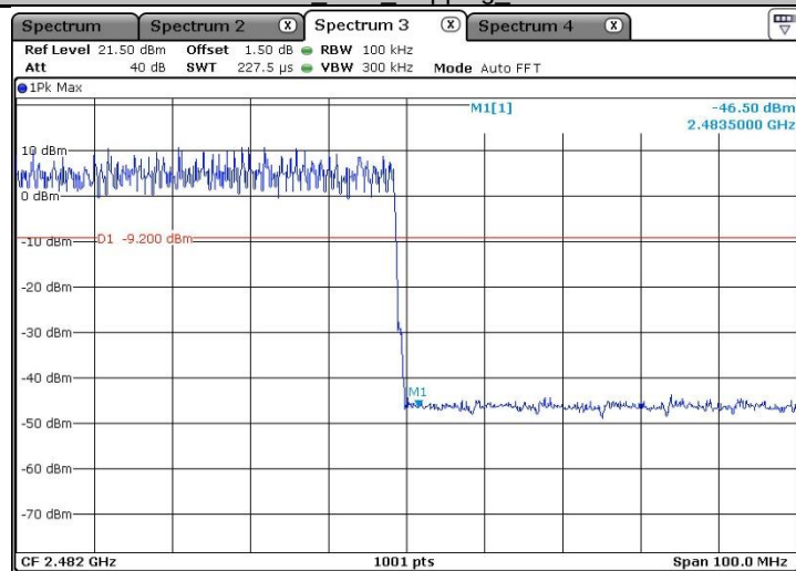
3DH5 Ant1 Hopping 2480
