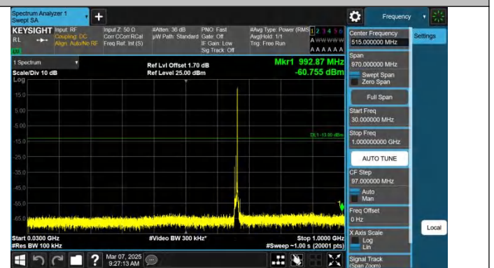
Band71-10MHz-QPSK-133172-1RB#49-30~1000-PASS
