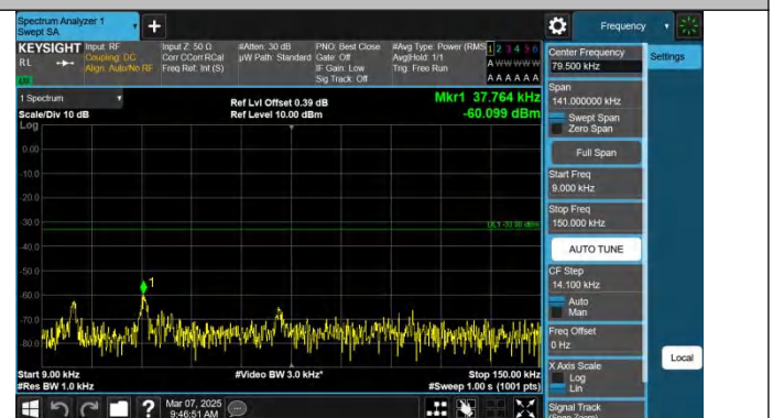
Band71-15MHz-QPSK-133397-1RB#74-0.009~0.15-PASS
