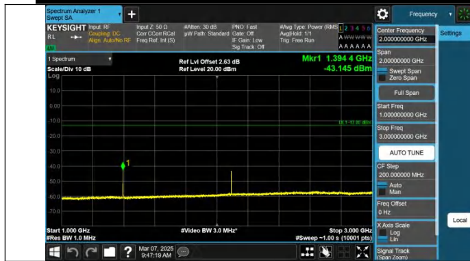
Band 71-15MHz-QPSK-133397-1RB#74-1000~3000-PASS
