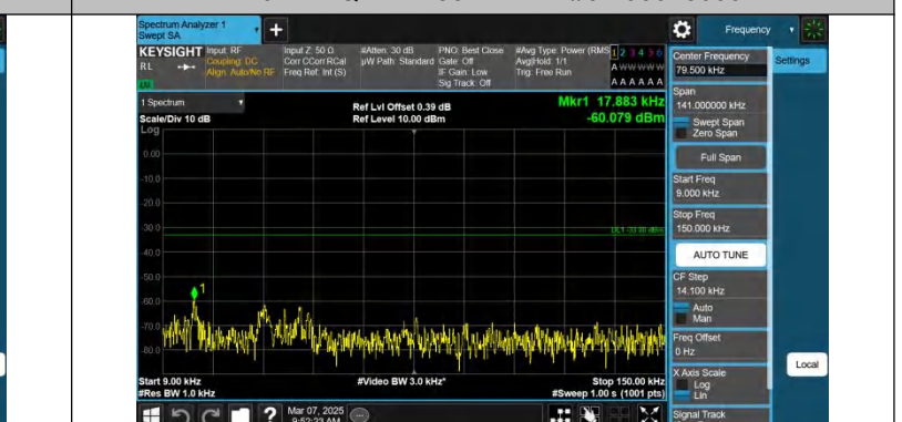
Band 71-20MHz-QPSK-133222-1RB#99-0.009~0.15-PASS
