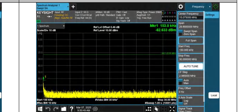
Band 71-20MHz-QPSK-133222-1RB#0-0.15~30-PASS
