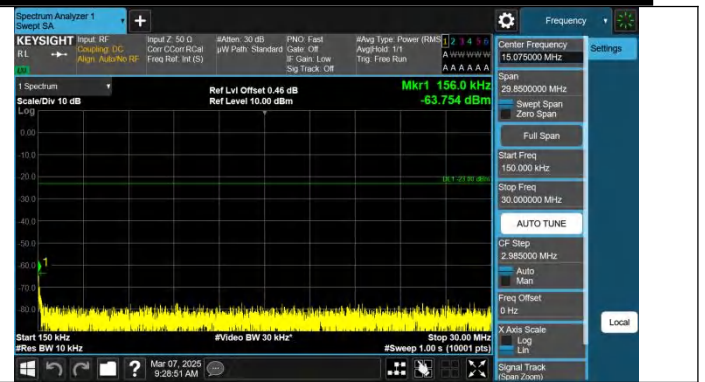
Band71-10MHz-QPSK-133297-1RB#0-0.15~30-PASS
