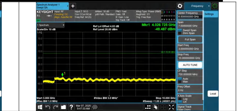
Band 71-15MHz-QPSK-133397-1RB#74-3000~10000-PASS
