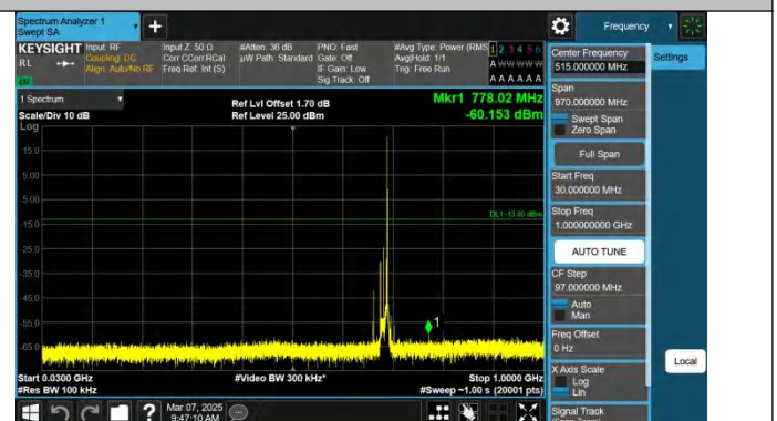
Band71-15MHz-QPSK-133397-1RB#74-30~1000-PASS
