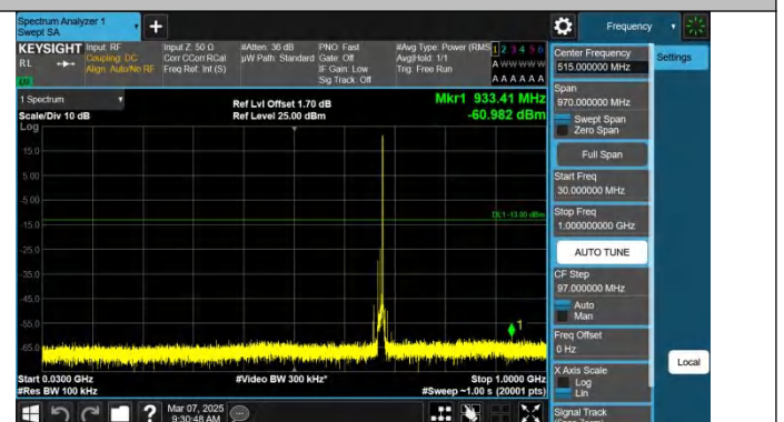
Band71-10MHz-QPSK-133297-1RB#49-30~1000-PASS
