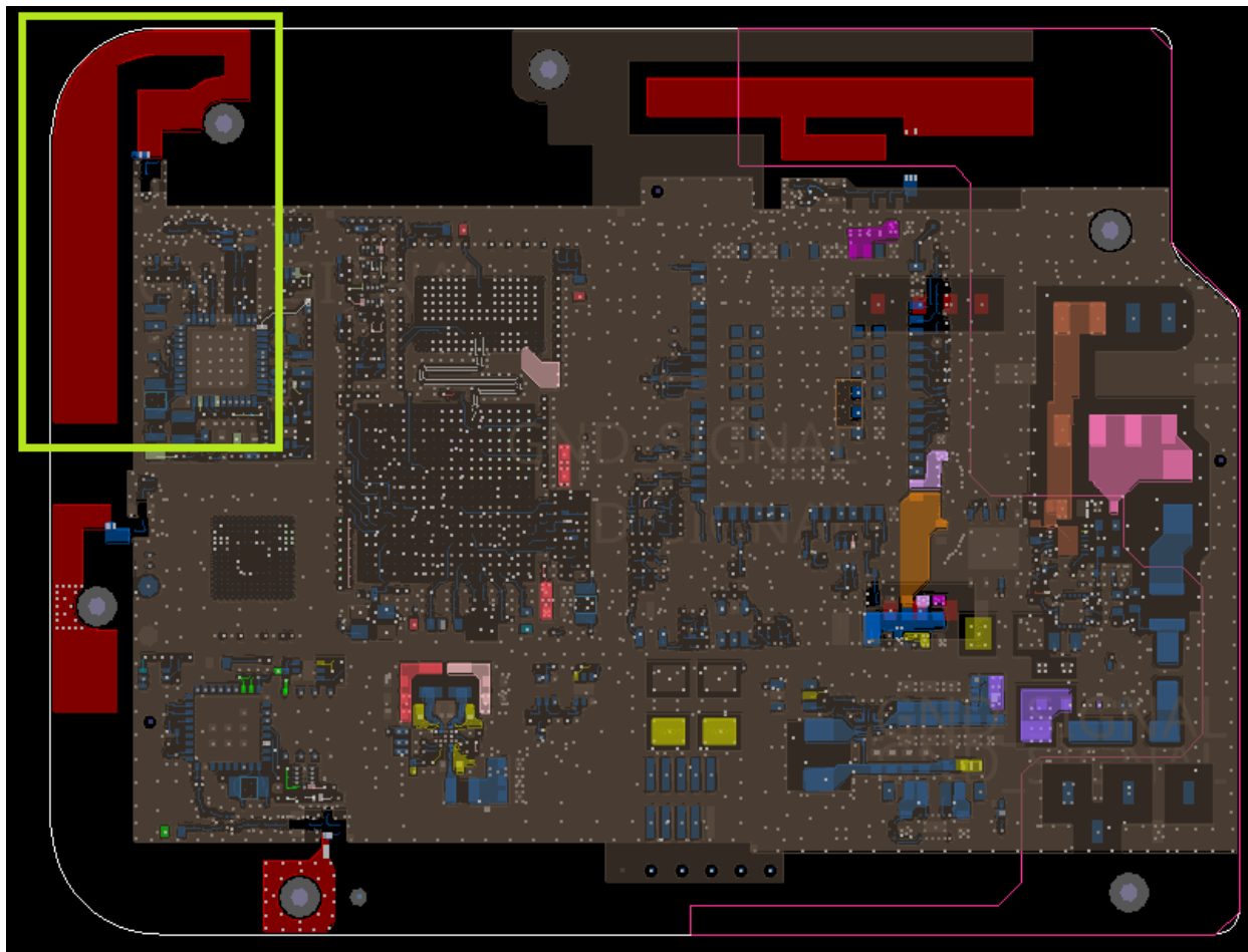
Figure 1. B014 PCB Antenna PCB-63695-003_reva
