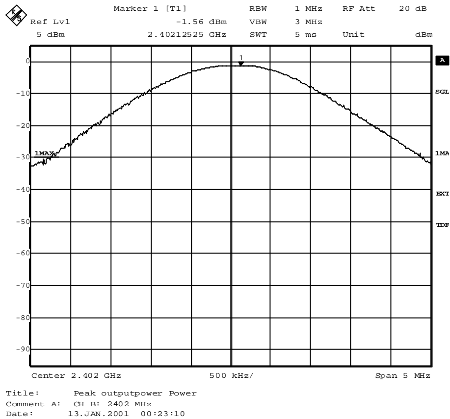
Peak output power (TX on 2402 MHz)
