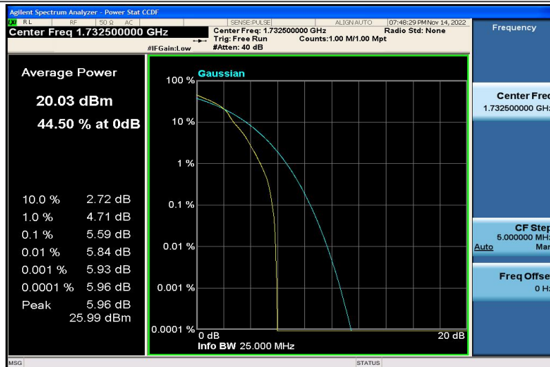
Band4-5MHz-16QAM-20175-1RB#0
