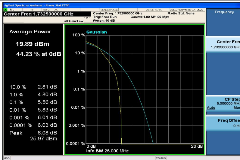
Band4-10MHz-16QAM-20175-1RB#0
