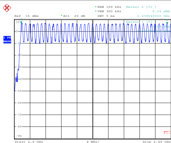
Plot 2
