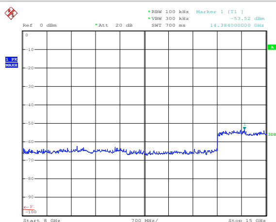
Plot 5 (8÷15GHz)
