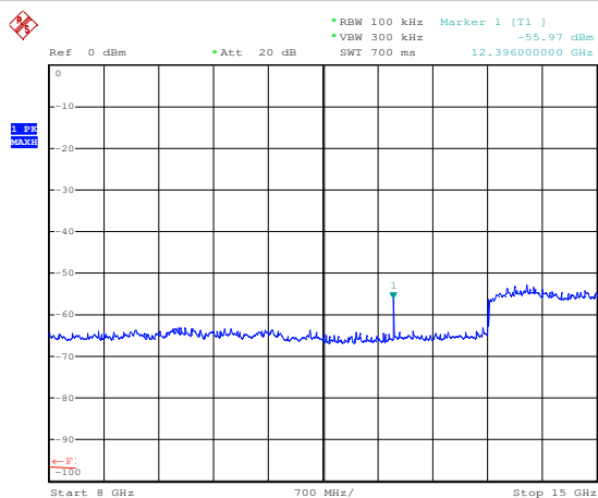
Plot 5 (8÷15GHz)
