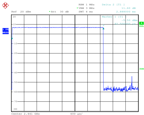
Plot 5 (DH5 packet)
