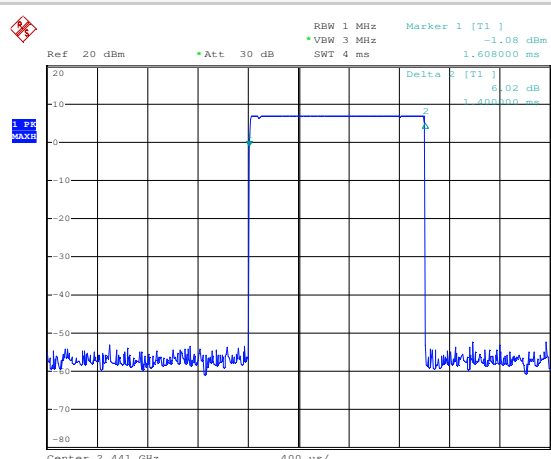
Plot 3 (DH3 packet)
