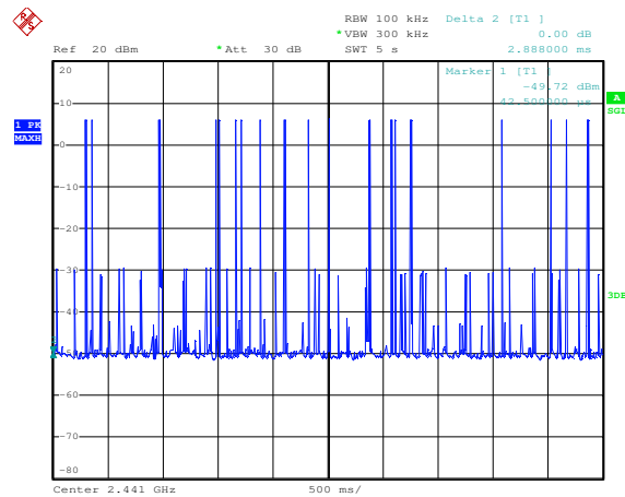
Plot 6 (DH5 packet) – N° of packets in 5s. (18 hops)
