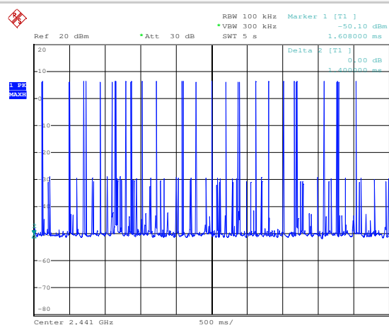
Plot 4 (DH3 packet) – N° of packets in 5s. (28 hops)
