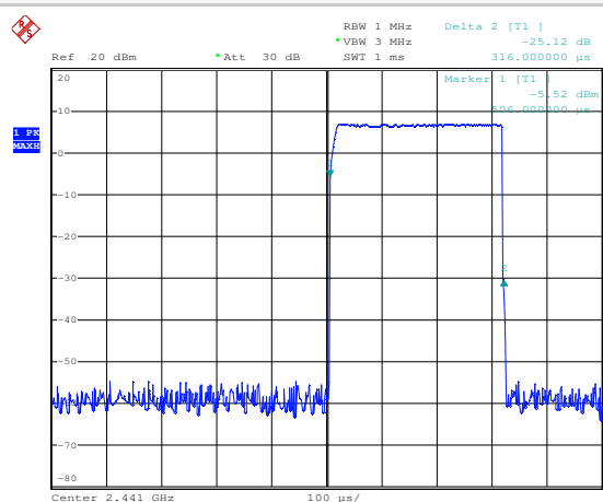
Plot 1 (DH1 packet)
