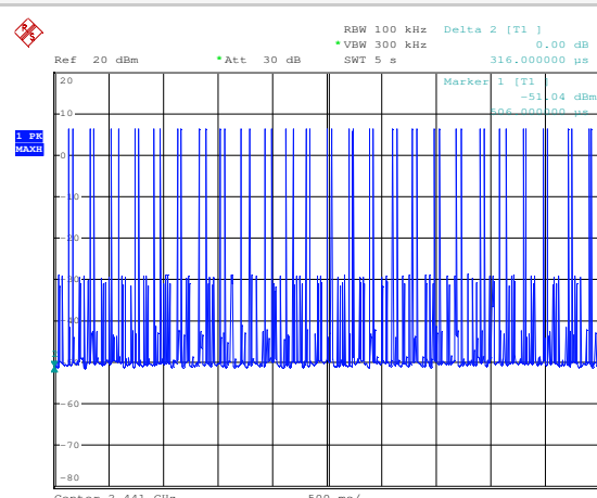
Plot 2 (DH1 packet) – N° of packets in 5s. (50 hops)
