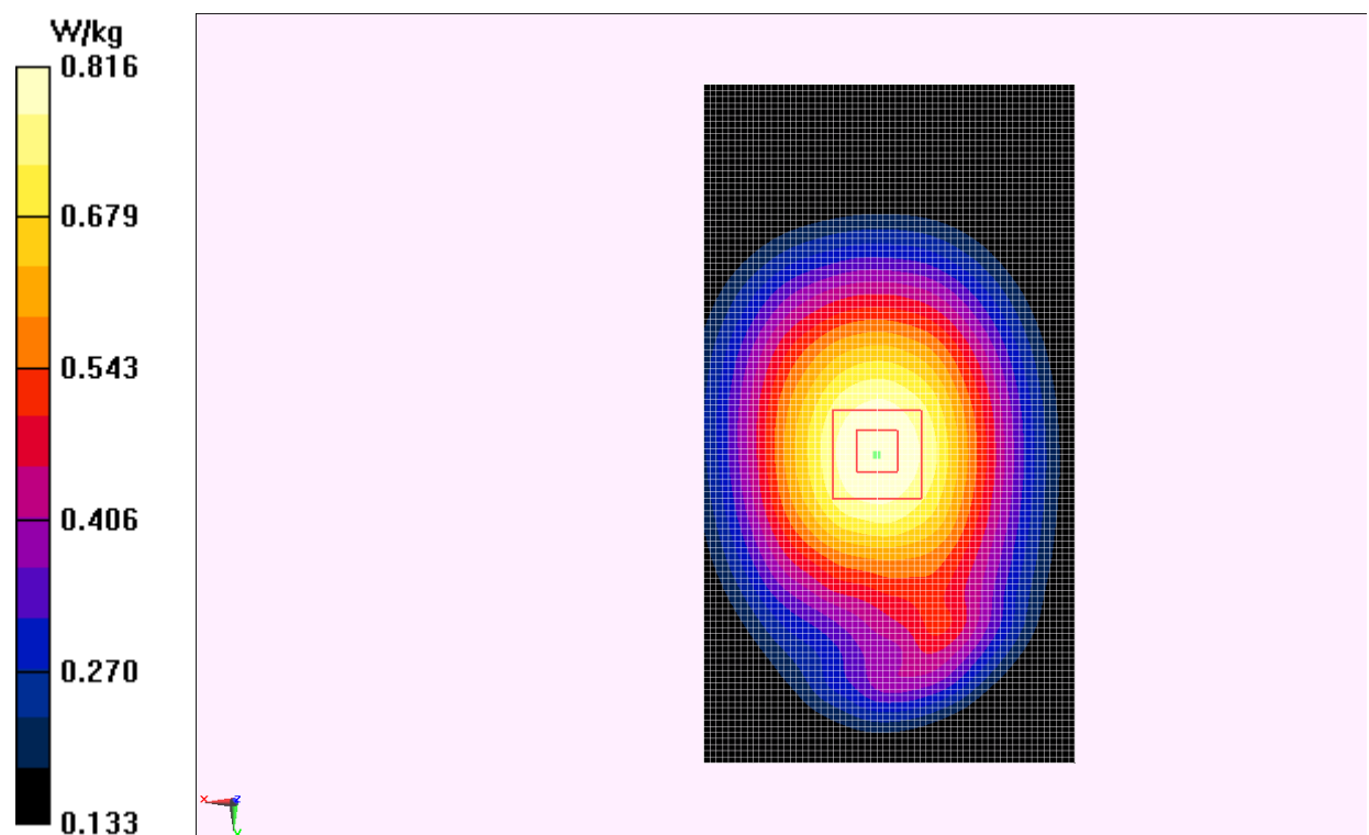
Fig.I.6 WCDMA 850 CH4182
