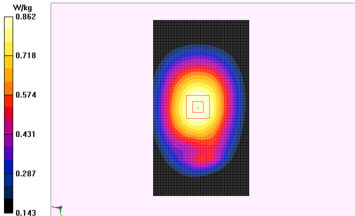
Fig.I.2 850 MHz CH128
