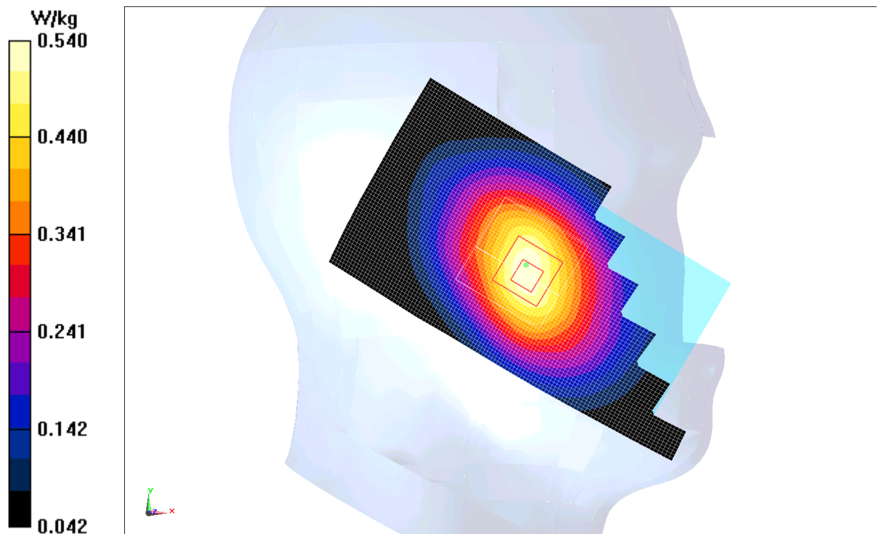
Fig.I.5 WCDMA 850 CH4233
