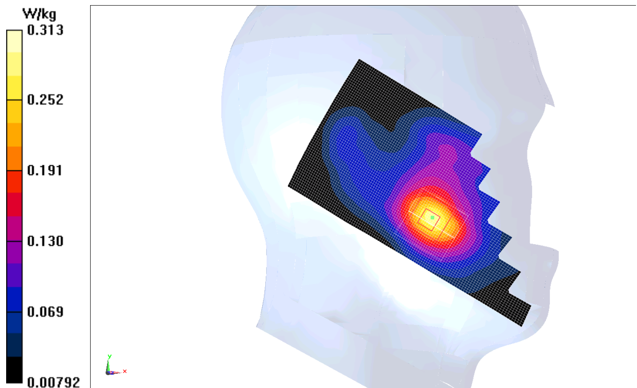
Fig.I.3 1900 MHz CH810
