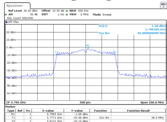
802.11ac40_5795MHz_Chain 1
