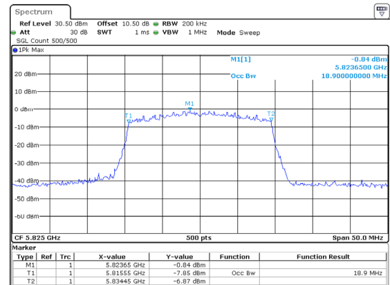
802.11ax20_5825MHz_RU_Full_Chain 2
