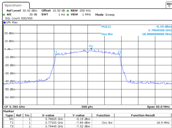
802.11ax20_5785MHz_RU_Full_Chain 2
