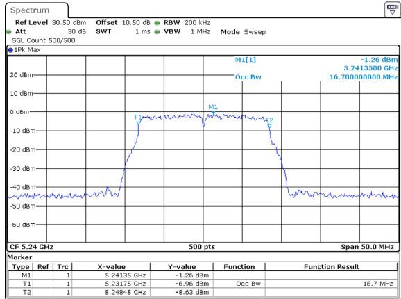
802.11a_5240MHz_Chain 2
