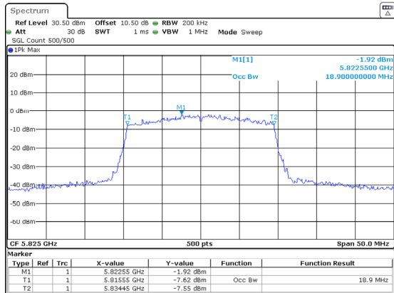
802.11ax20_5825MHz_RU_Full_Chain 1
