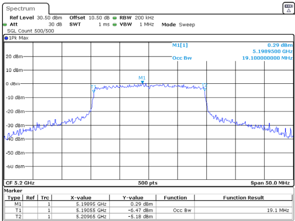
802.11ax20_5200MHz_RU_Full_Chain 1
