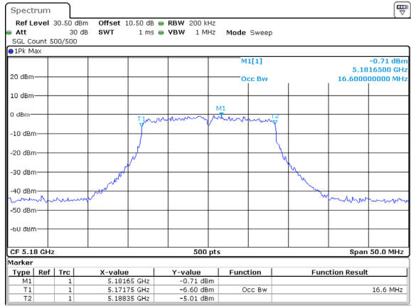
802.11a_5180MHz_Chain 2
