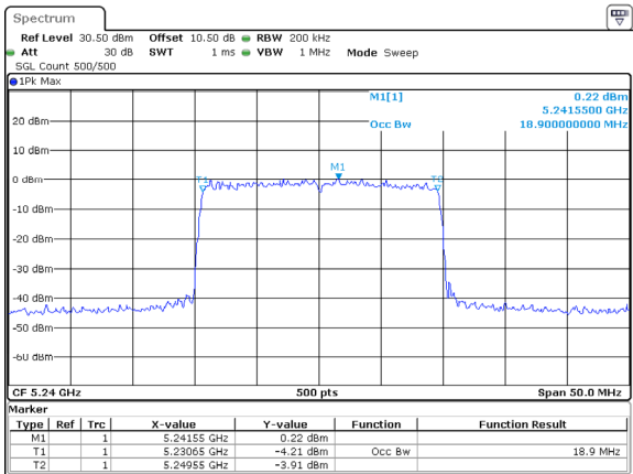
802.11ax20_5240MHz_RU_Full_Chain 2
