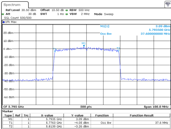
802.11ax40_5795MHz_RU_Full_Chain 2
