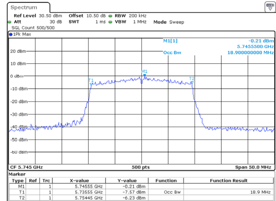
802.11ax20_5745MHz_RU_Full_Chain 2
