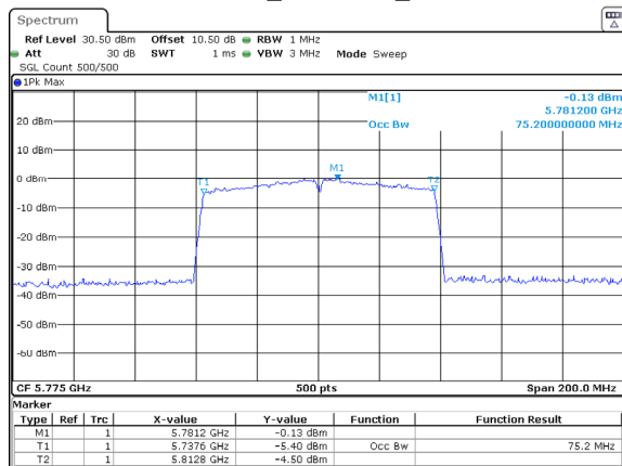
802.11ac80_5775MHz_Chain 1
