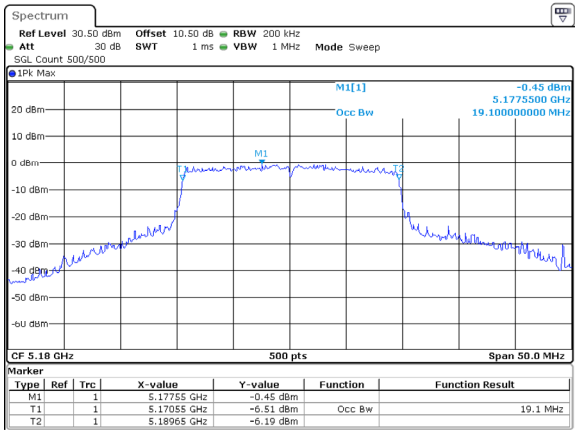
802.11ax20_5180MHz_RU_Full_Chain 2
