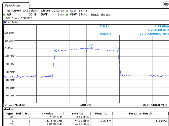
802.11ac80_5775MHz_Chain 2
