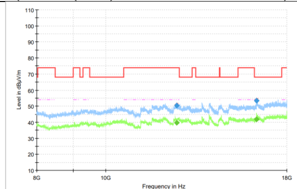
Radiated Spurious Emission (802.11ax(HE20)MIMO, ch229, 8GHz-18GHz)
