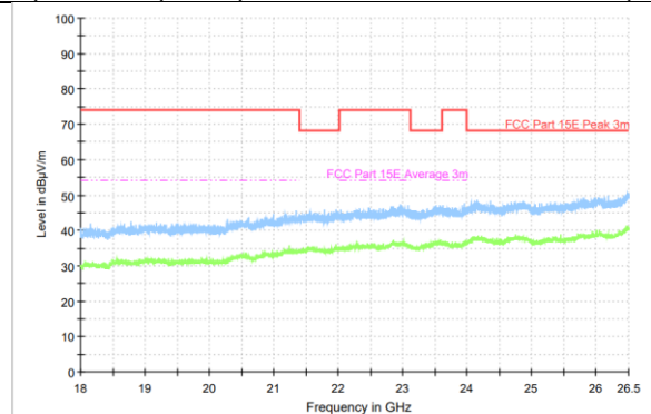
Radiated Spurious Emission (802.11ax(HE40)MIMO, ch3, 18GHz-26.5GHz)
