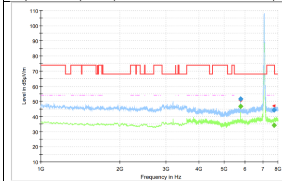
Radiated Spurious Emission (802.11ax(HE20)MIMO, ch229, 1GHz-8GHz)
