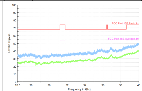
Radiated Spurious Emission (802.11ax(HE80)MIMO, ch215, 26.5GHz-40GHz)
