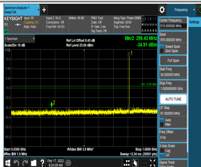
Band26-5MHz-QPSK-26715-1-0-Low-30-1000--34.91-PASS
