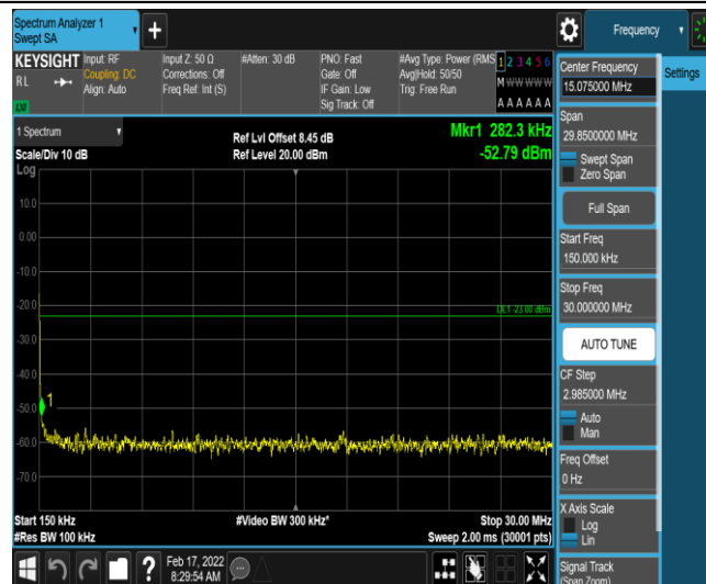
Band26-5MHz-QPSK-26765-1-0-High-0.15-30--52.79-PASS
