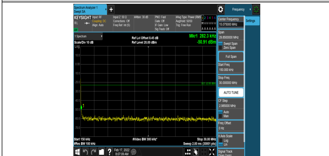
Band26-1.4MHz-16QAM-26783-1-0-High-0.15-30--50.91-PASS
