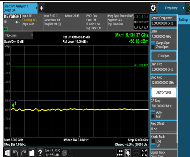
Band26-3MHz-16QAM-26740-1-0-Low-5000-12000--58.18-PASS
