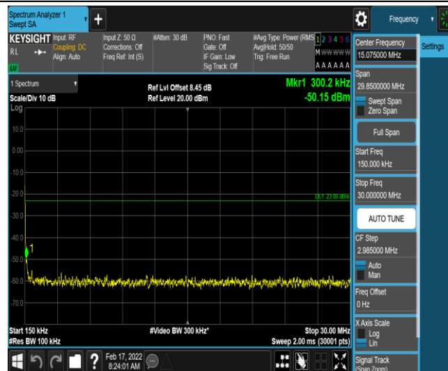
Band26-5MHz-QPSK-26715-1-0-Low-0.15-30--50.15-PASS
