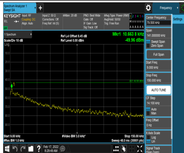
Band26-5MHz-QPSK-26765-1-0-High-0.009-0.15--49.96-PASS
