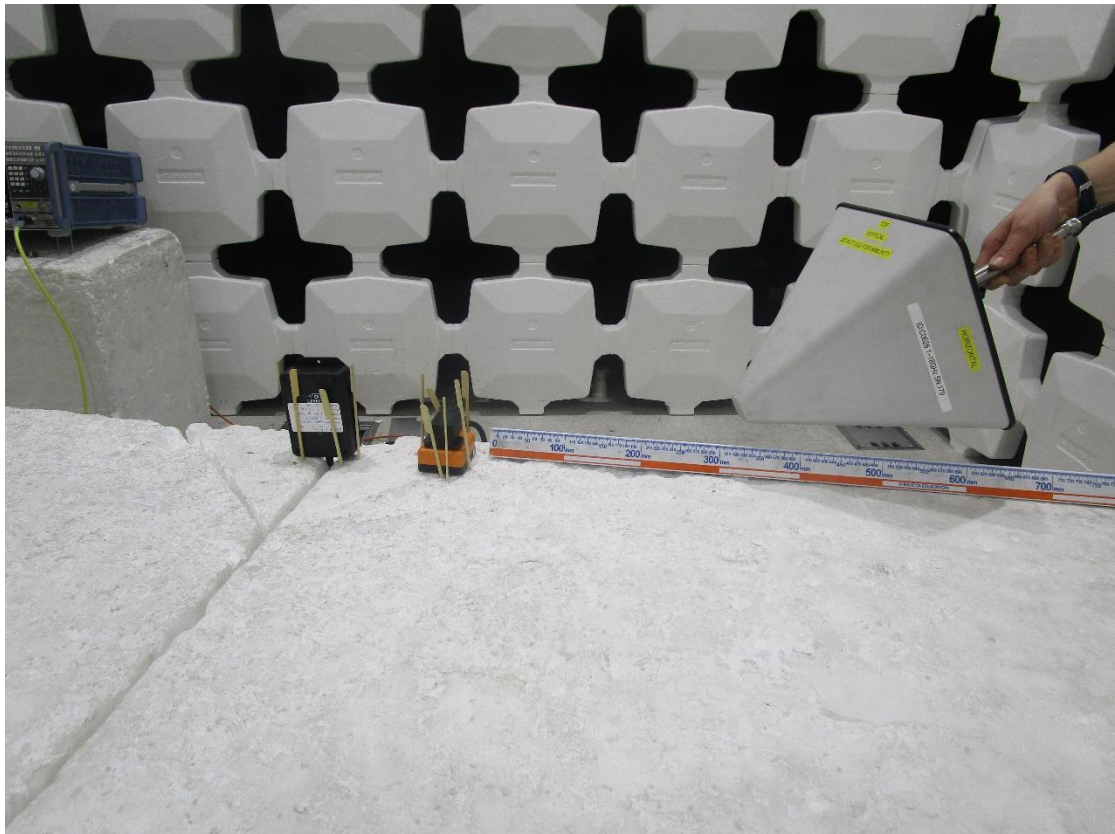
Exploratory emissions 1GHz to 18GHz
