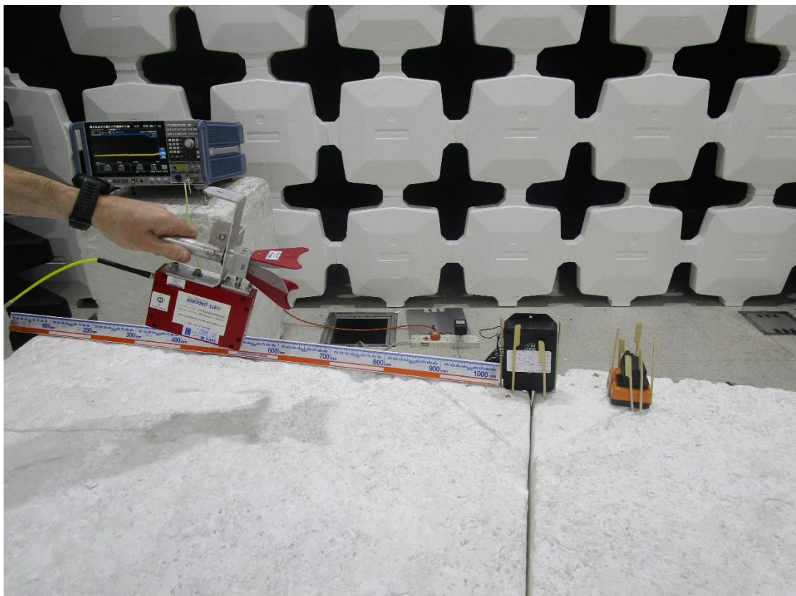
Exploratory emissions 18GHz to 25GHz
