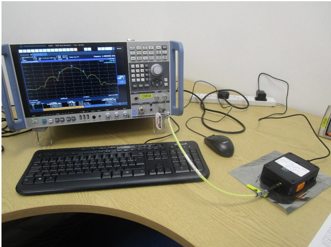
Arrangements for conducted tests
