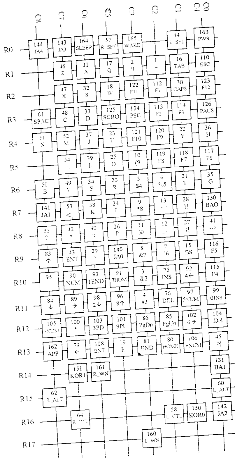
Fig. 6.1 Keyboard Matrix
