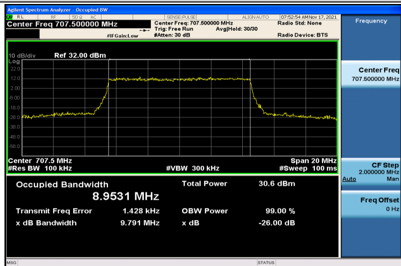
Band12-10MHz-16QAM-23095-50RB#0-8.9531
