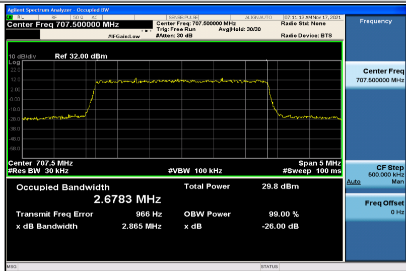
Band12-3MHz-16QAM-23095-15RB#0-2.6783
