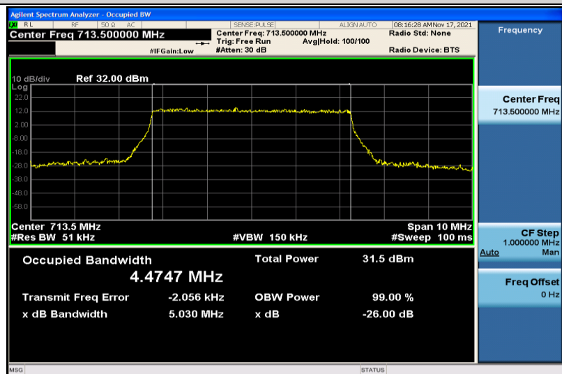
Band17-5MHz-QPSK-23825-25RB#0-4.4747
