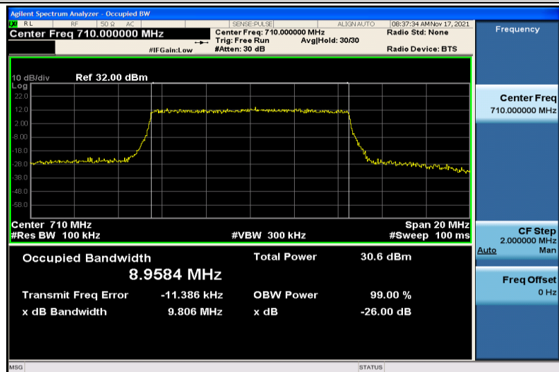
Band17-10MHz-16QAM-23790-50RB#0-8.9584
