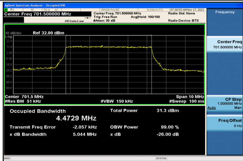
Band12-5MHz-QPSK-23035-25RB#0-4.4729
