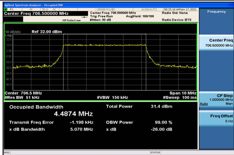
Band17-5MHz-QPSK-23755-25RB#0-4.4874
