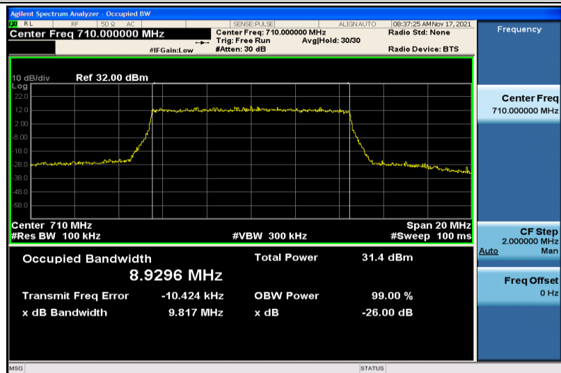
Band17-10MHz-QPSK-23790-50RB#0-8.9296
