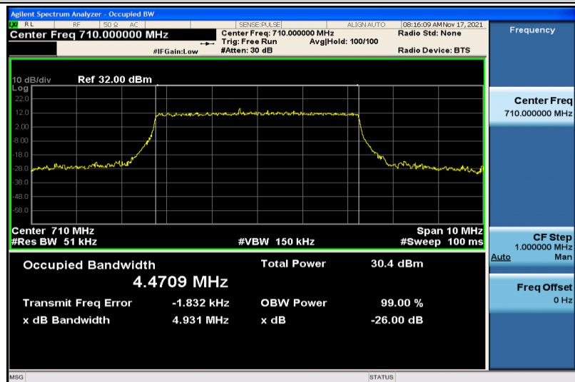
Band17-5MHz-16QAM-23790-25RB#0-4.4709
