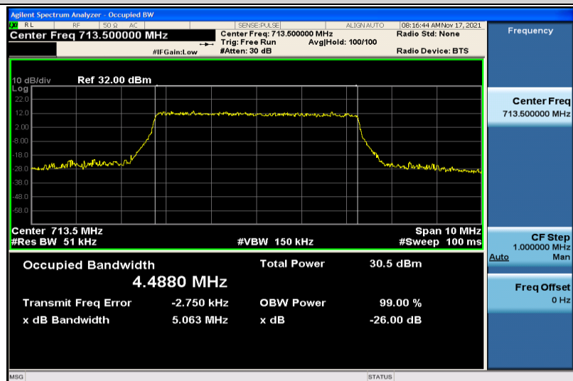
Band17-5MHz-16QAM-23825-25RB#0-4.4880
