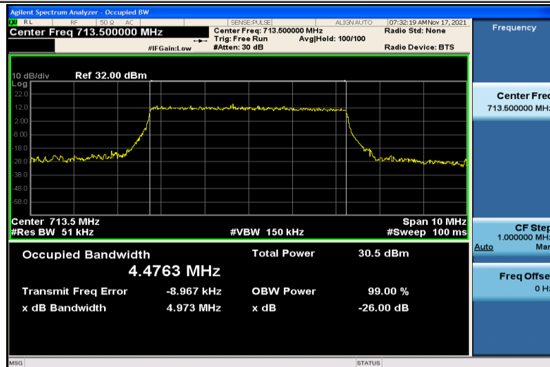
Band12-5MHz-16QAM-23155-25RB#0-4.4763
