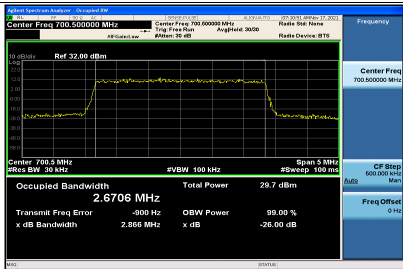
Band12-3MHz-16QAM-23025-15RB#0-2.6706
