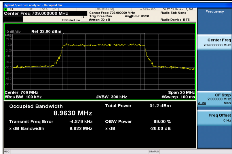
Band17-10MHz-QPSK-23780-50RB#0-8.9630
