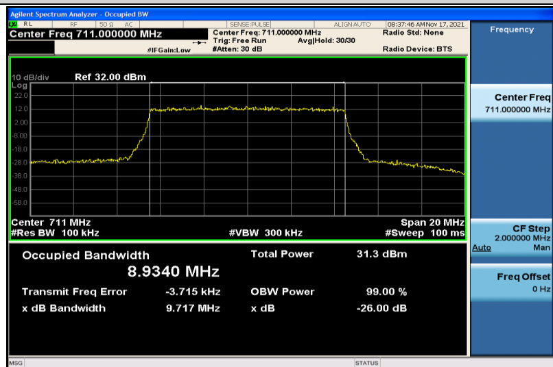
Band17-10MHz-QPSK-23800-50RB#0-8.9340
