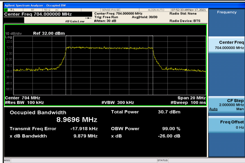
Band12-10MHz-16QAM-23060-50RB#0-8.9696
