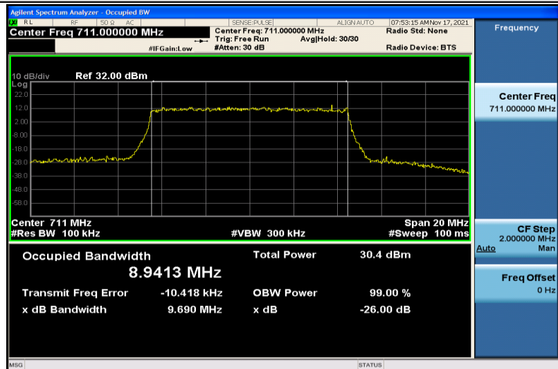
Band12-10MHz-16QAM-23130-50RB#0-8.9413
