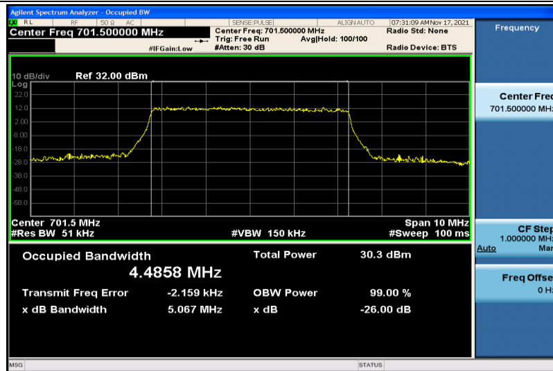
Band12-5MHz-16QAM-23035-25RB#0-4.4858
