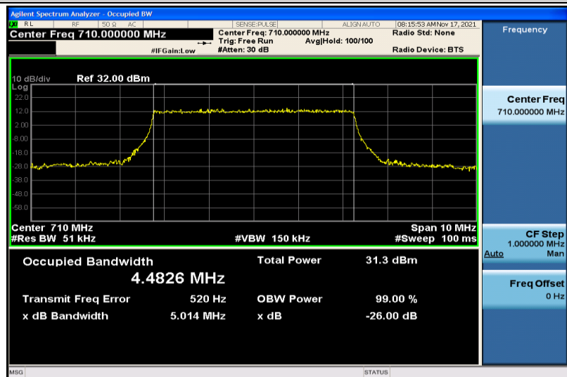
Band17-5MHz-QPSK-23790-25RB#0-4.4826
