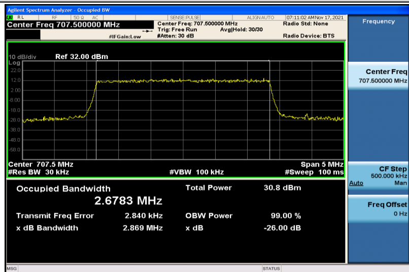
Band12-3MHz-QPSK-23095-15RB#0-2.6783
