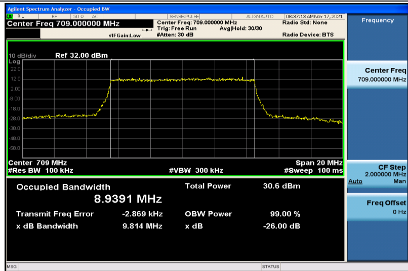
Band17-10MHz-16QAM-23780-50RB#0-8.9391
