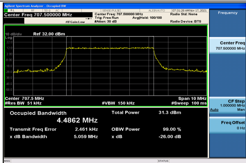
Band12-5MHz-QPSK-23095-25RB#0-4.4862
