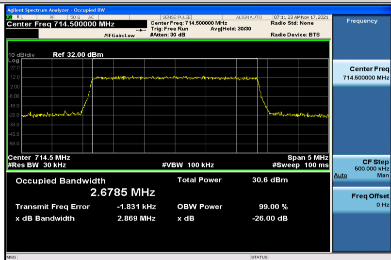
Band12-3MHz-QPSK-23165-15RB#0-2.6785
