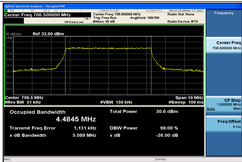
Band17-5MHz-16QAM-23755-25RB#0-4.4845
