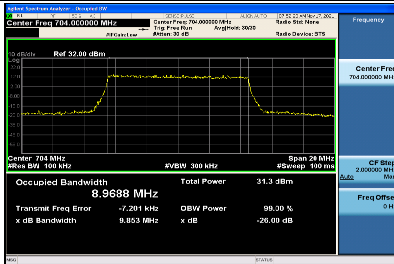
Band12-10MHz-QPSK-23060-50RB#0-8.9688
