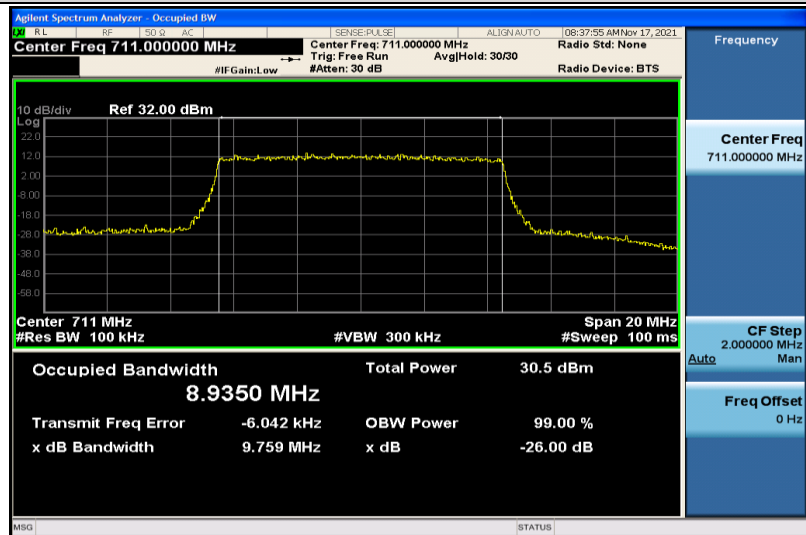
Band17-10MHz-16QAM-23800-50RB#0-8.9350
