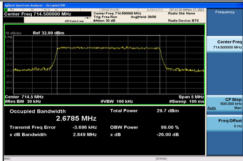
Band12-3MHz-16QAM-23165-15RB#0-2.6785
