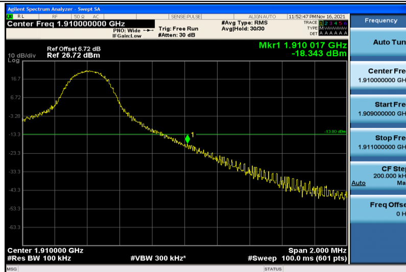
Band2-10MHz-QPSK-19150-1RB#49
