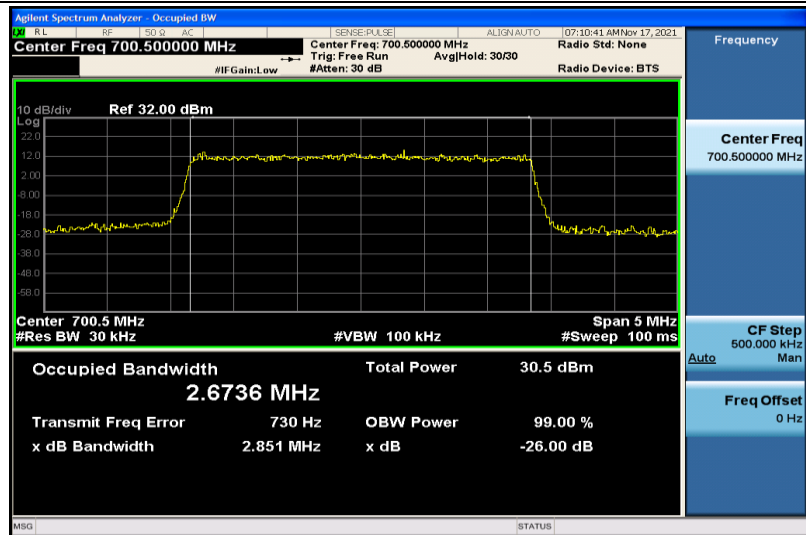
Band12-3MHz-QPSK-23025-15RB#0-2.6736
