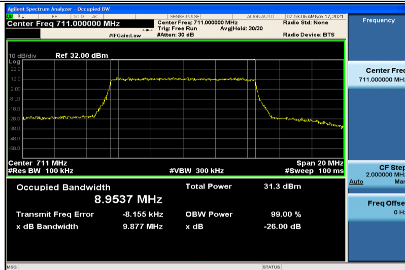
Band12-10MHz-QPSK-23130-50RB#0-8.9537
