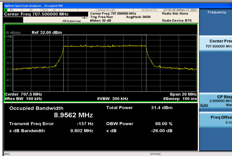
Band12-10MHz-QPSK-23095-50RB#0-8.9562
