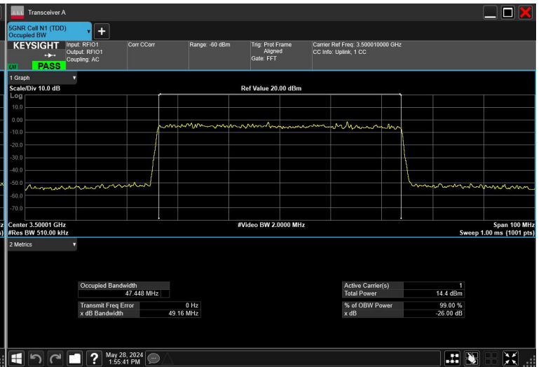
50MHz_30kHz_3500MHz_CP-OFDM256QAM_RB133@0
