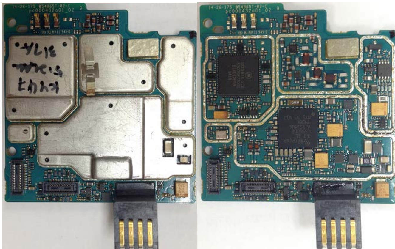
RF board with and without Shields (Top)
