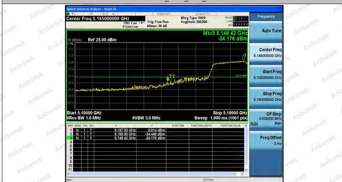
11N40SISO_Ant1_Low_5190
