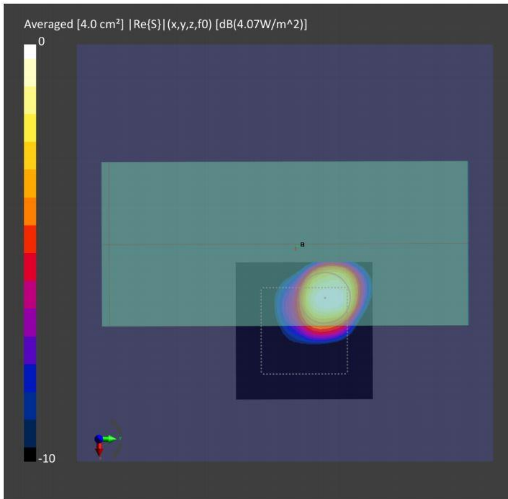
Figure 8-3: 4cm2-averaged power density distribution measured at input.power.limit of 2.68 dBm on the Back for n261 beam 19
