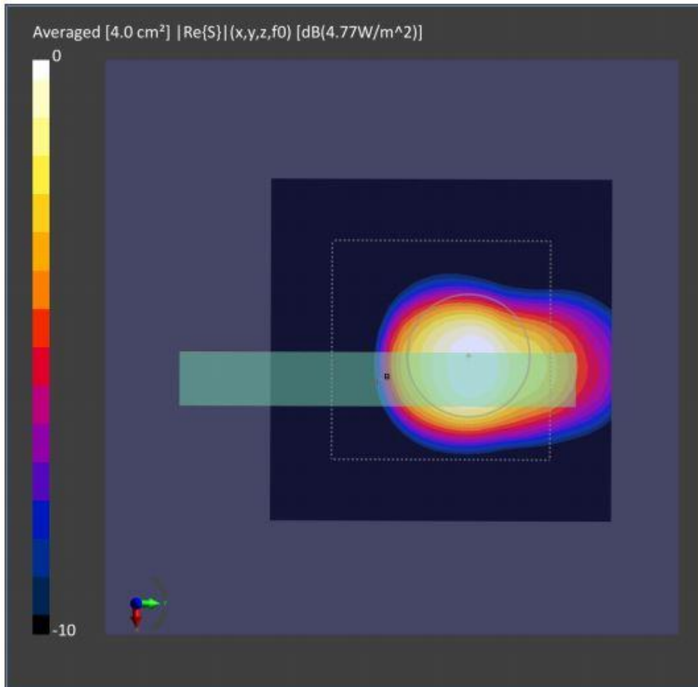
Figure 8-2: 4cm2-averaged power density distribution measured at input.power.limit of 1.69 dBm on the Right Side surface for n260 beam 23
